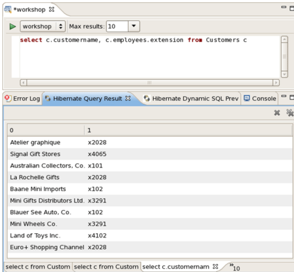
Figure 3.43. The Hibernate Query Result
