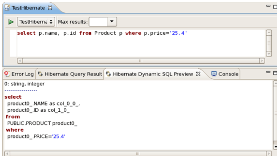
Figure 3.29. Hibernate Dynamic Query Translator View
