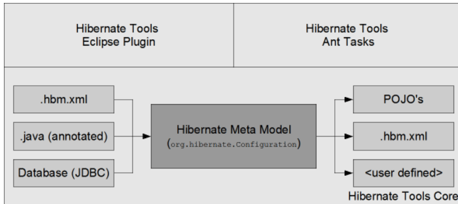
Figure 2.1. Hibernate Core Concepts
