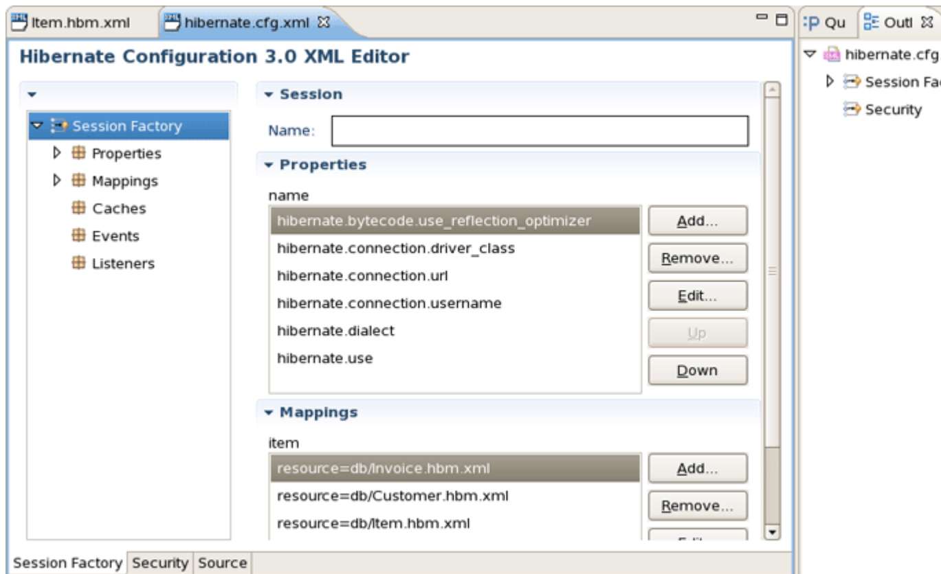
Figure 3.17. Structured cfg.xml Editor
