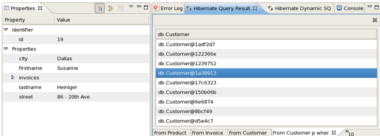
Figure 3.30. Properties View
