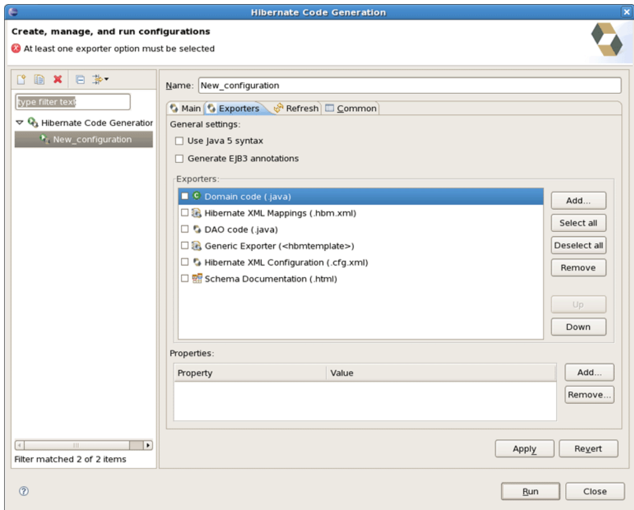
Figure 3.11. Selecting Exporters
