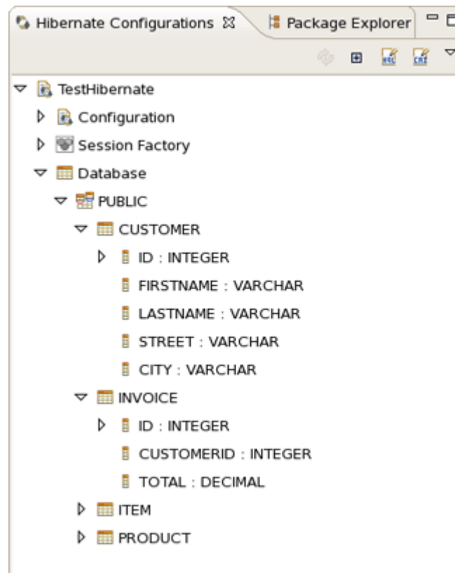
Figure 3.8. Console Overview
