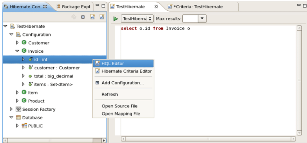
Figure 3.28. Entering Simple Queries
