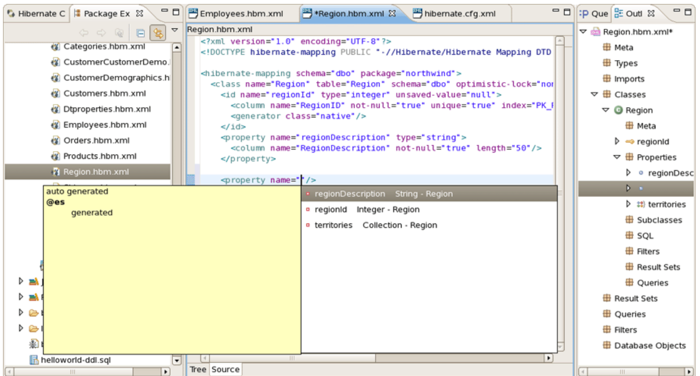
Figure 3.12. XML Editing Functionality
