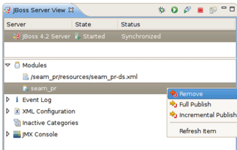
Figure 3.9. Modules Action
