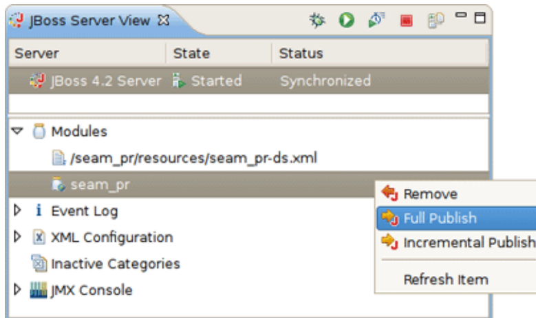
Figure 5.6. Full Publish
