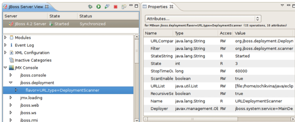
Figure 3.18. JMX Console
