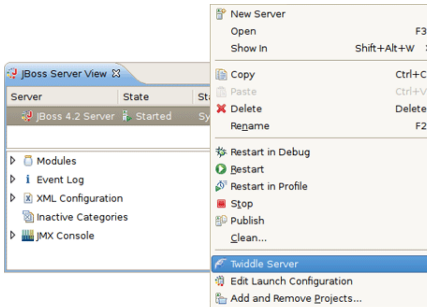
Figure 3.6. Twiddle Server
