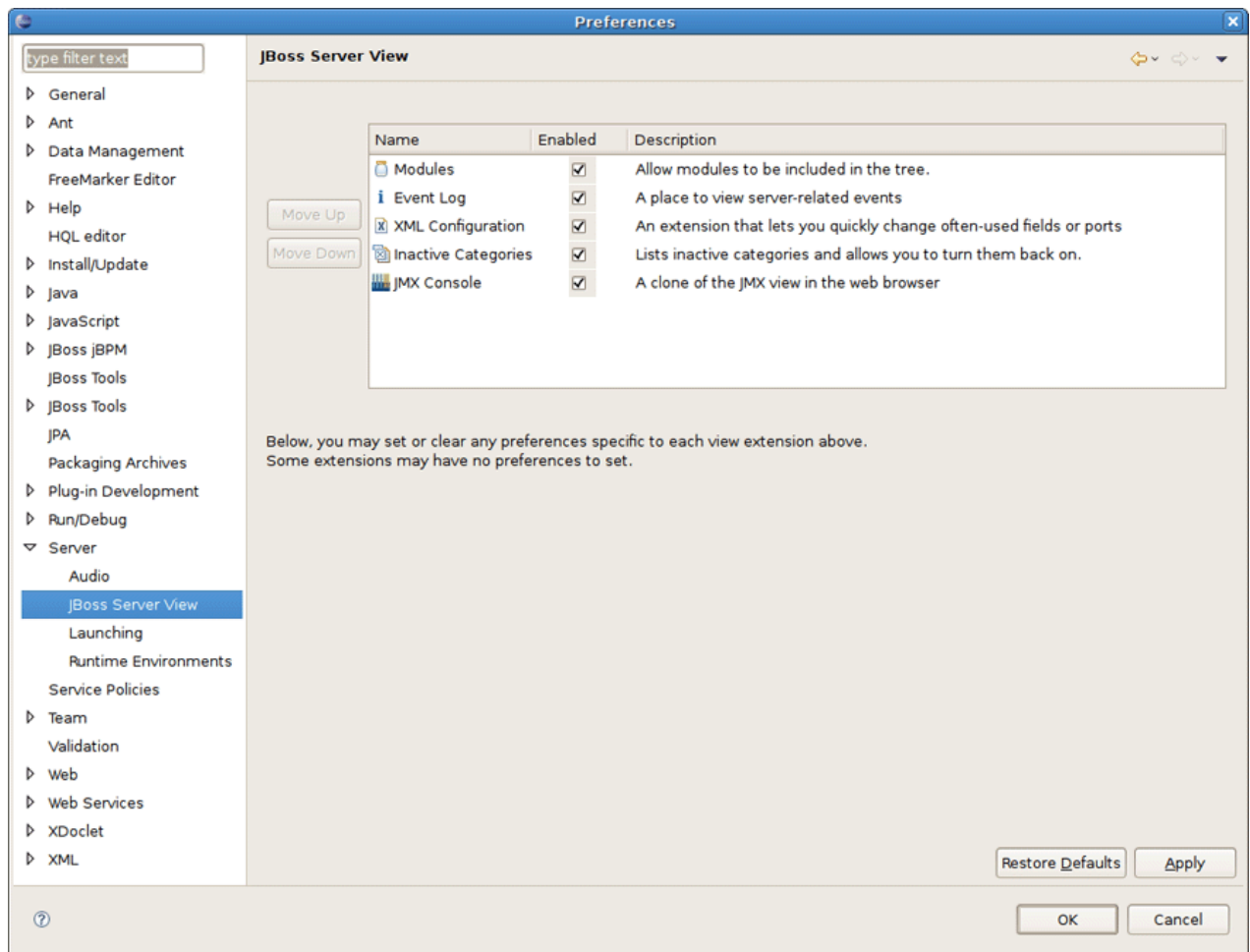
Figure 3.8. View Preferences
