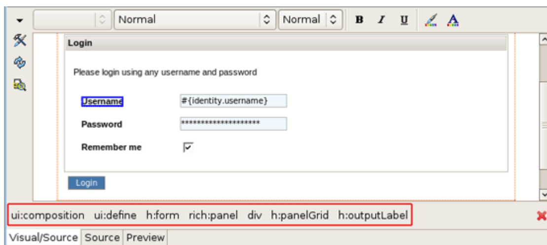
Figure 3.58. Selection Tag Bar
