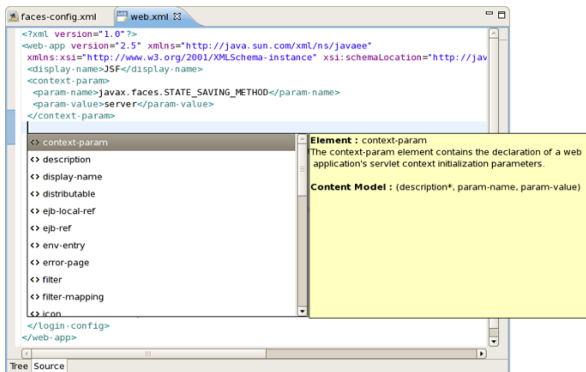
Figure 3.13. Content Assist in web.xml File
