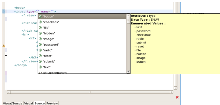
Figure 3.24. HTML Tags Content Assist
