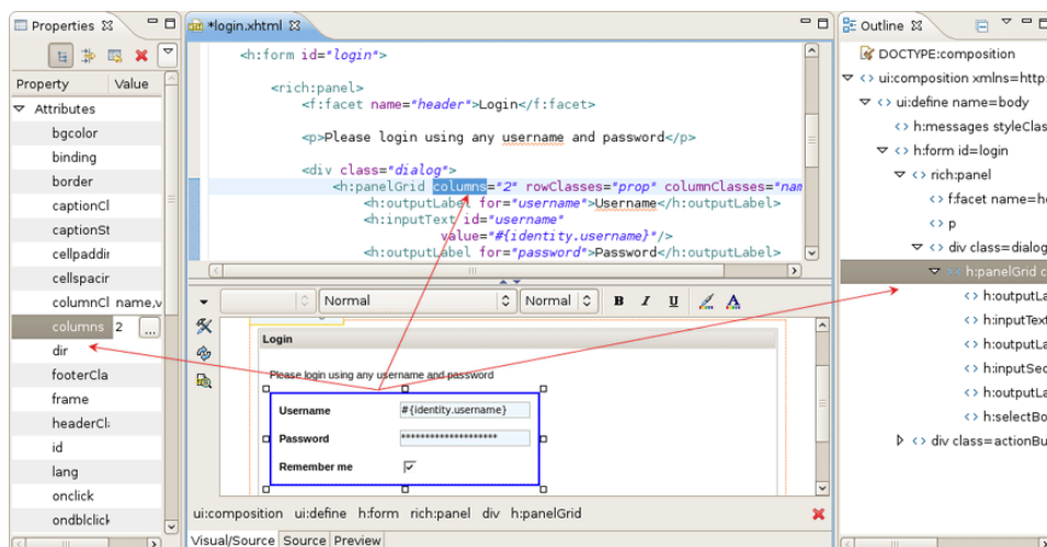
Figure 3.34. Integration with Properties and Outline Views
