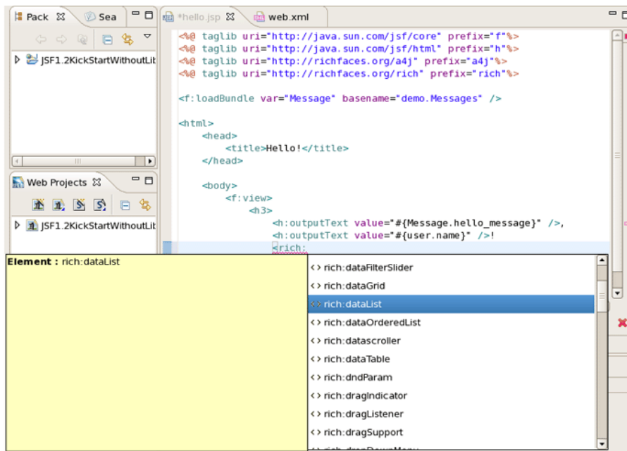
Figure 3.26. Content Assist for RichFaces Components
