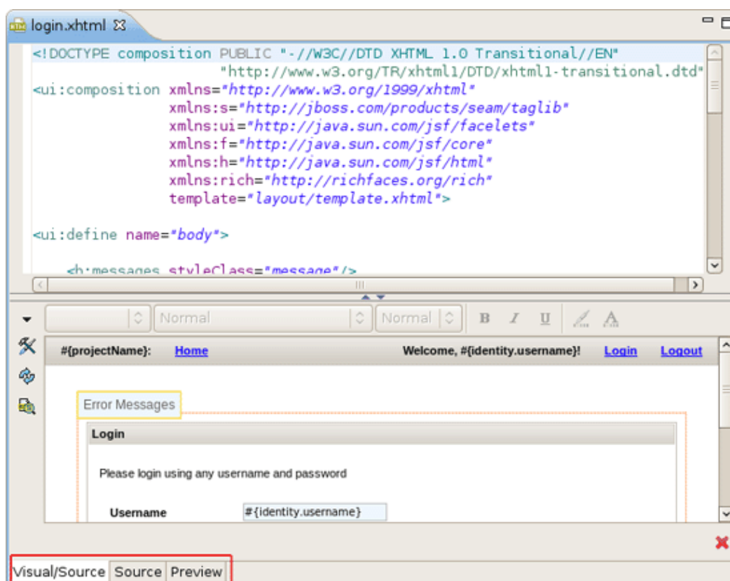
Figure 3.32. Visual Page Editor
