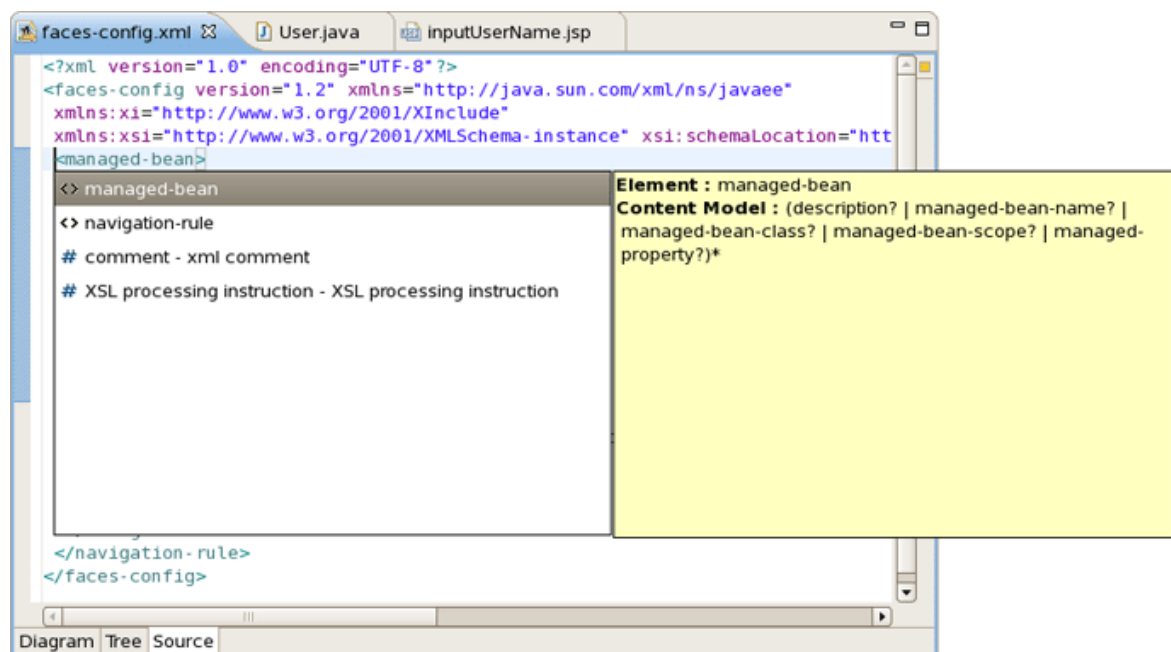
Figure 3.11. Content Assist in JSF Configuration File
