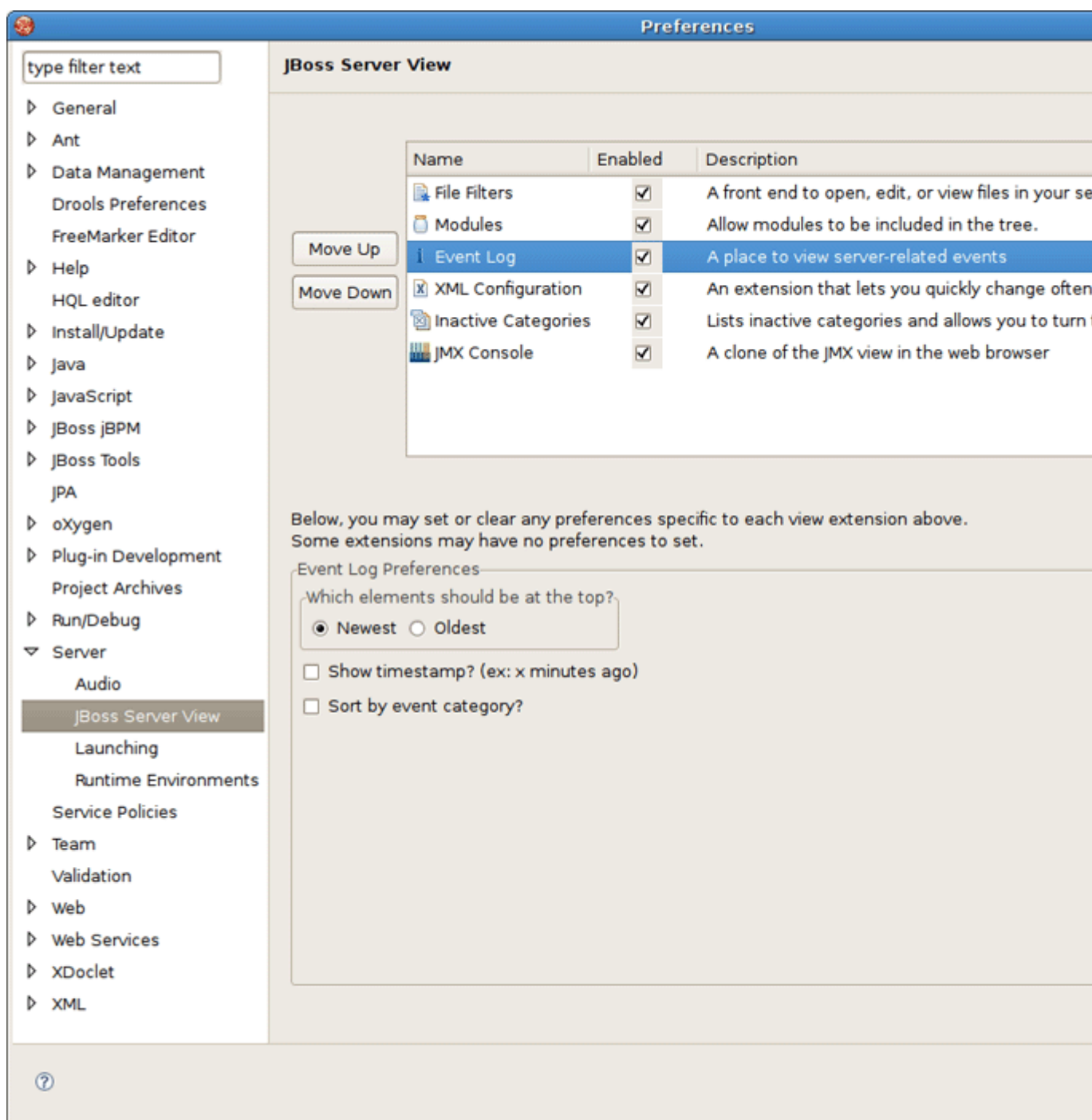
Figure 6.36. JBoss Server View Preferences
