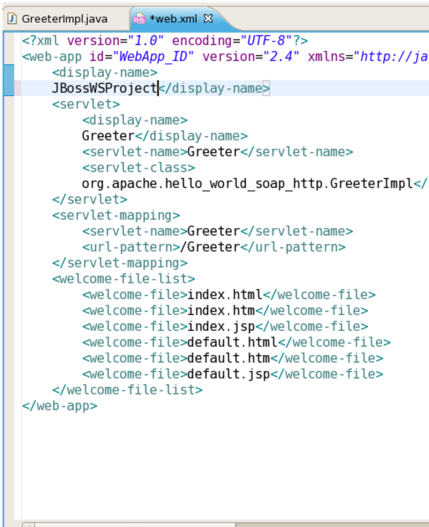
Figure 2.11. Web.xml
