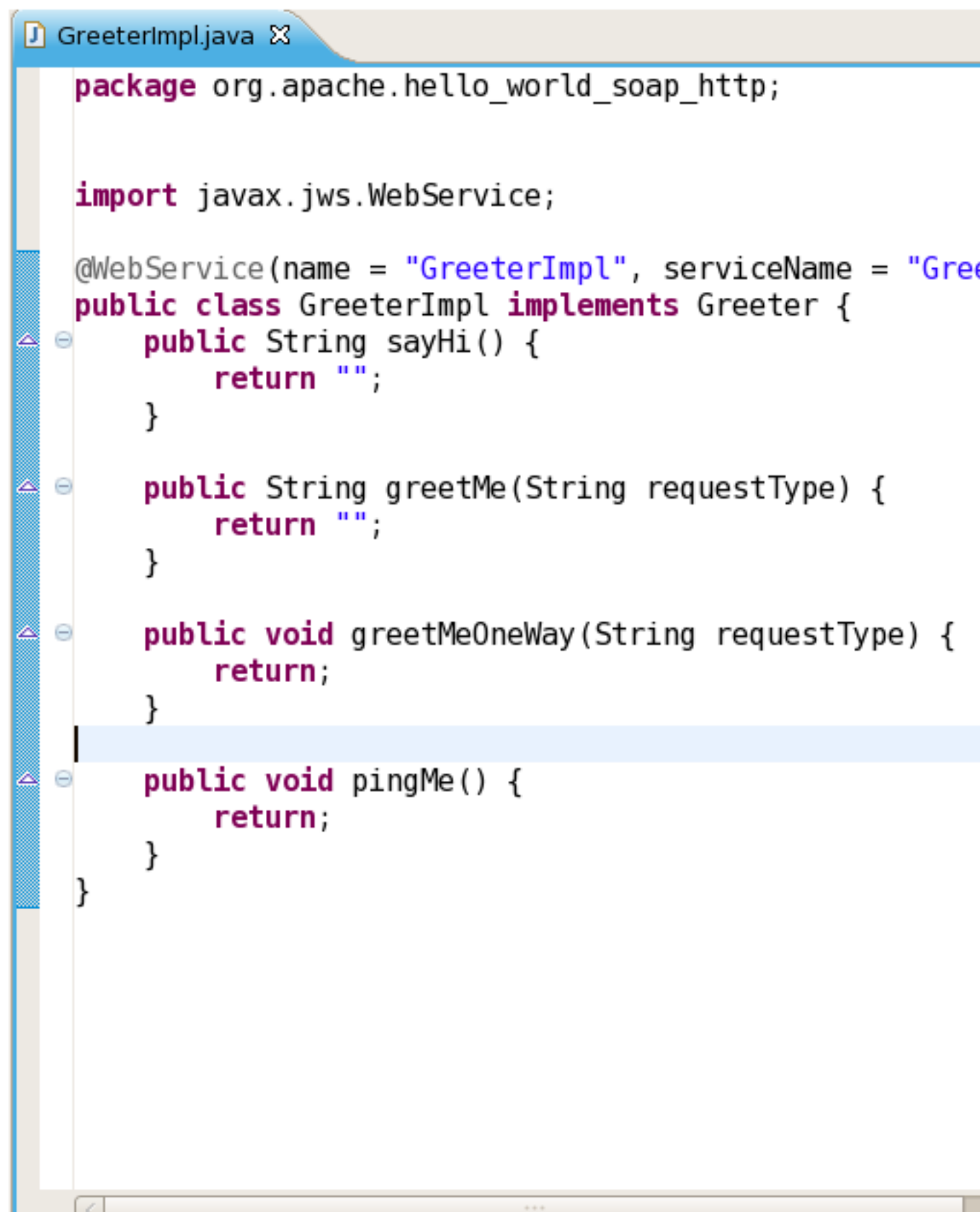
Figure 2.10. The generated implementation Java code
