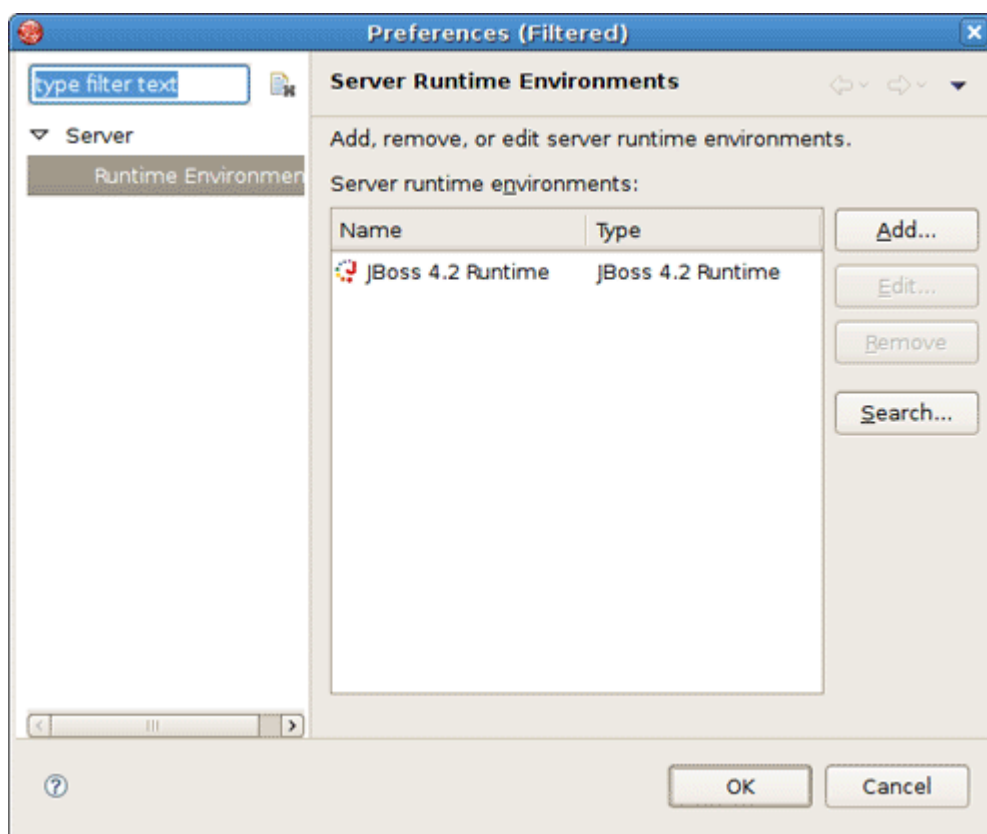
Figure 2.9. Installed Runtimes
