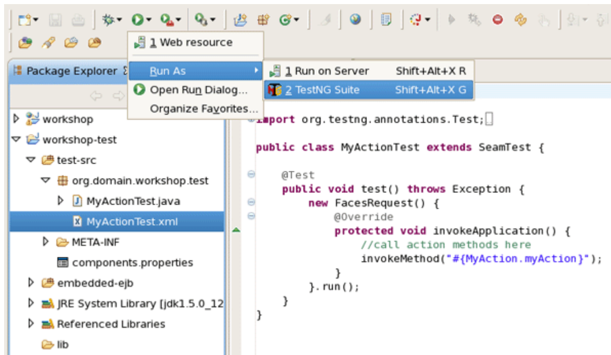
Figure 3.22. TestNG Running
