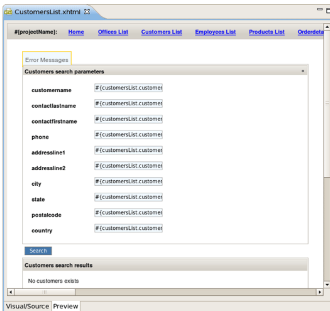
Figure 3.38. CustomersList.xhtml in the Editor
