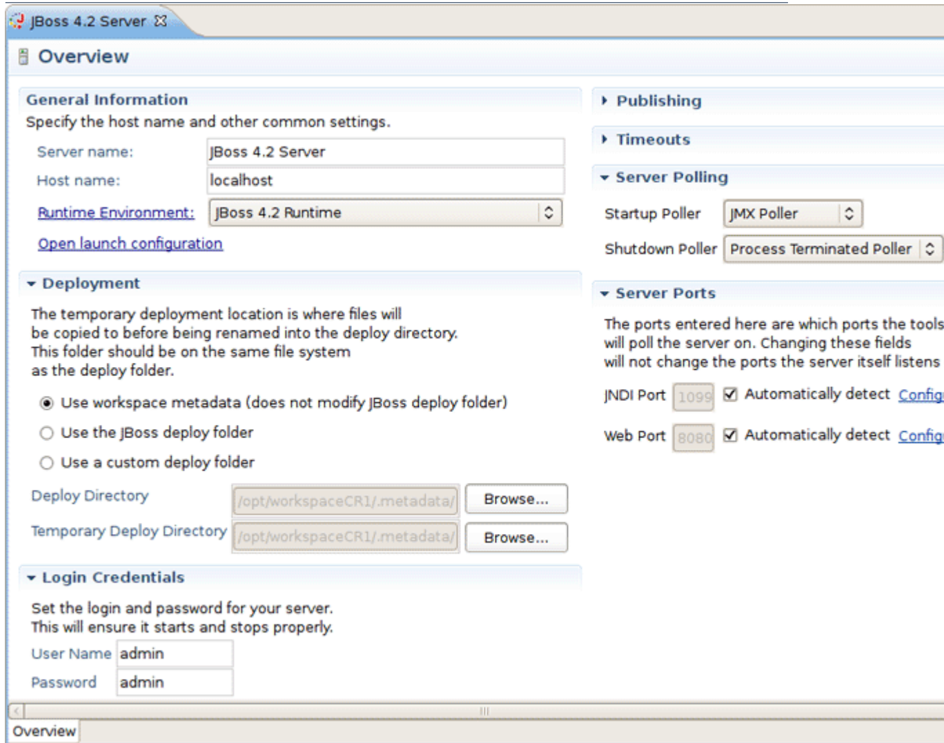
Figure 2.7. Server Overview
