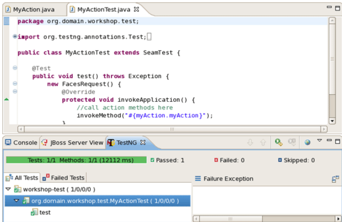
Figure 3.23. TestNG Results
