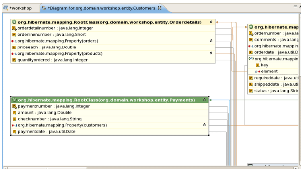
Figure 3.47. Diagram Tab
