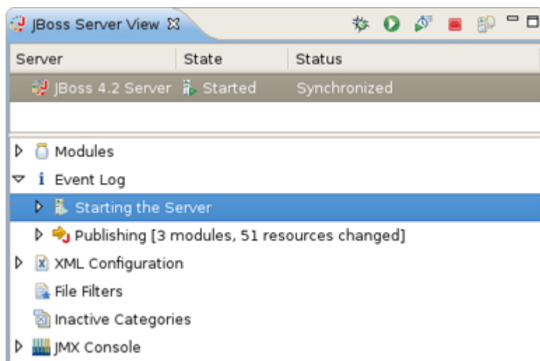
Figure 2.5. Event Log
