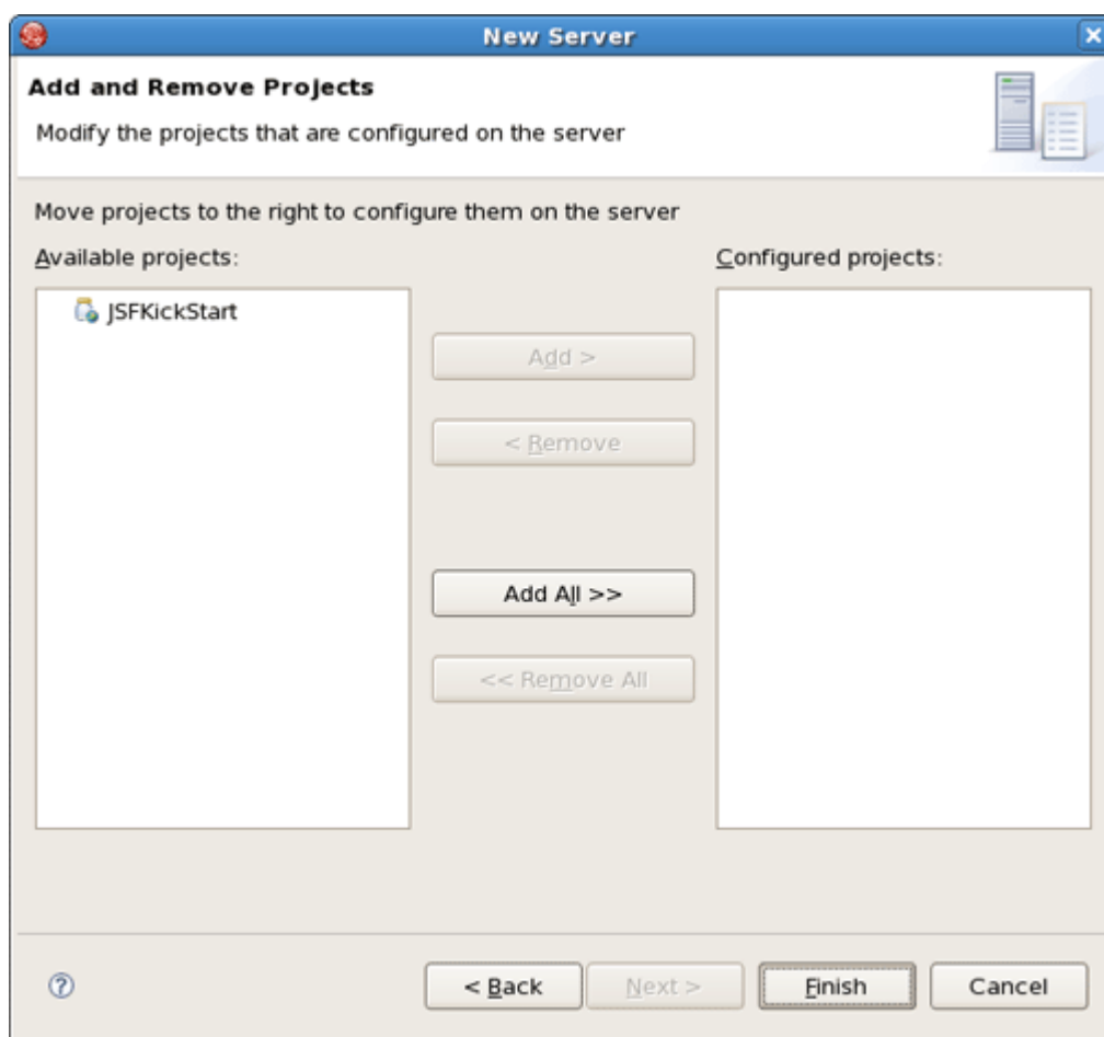
Figure 2.13. Configuring Projects
