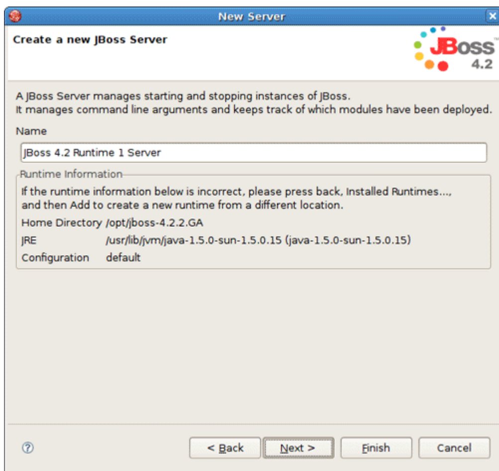
Figure 2.12. Configuring Projects
