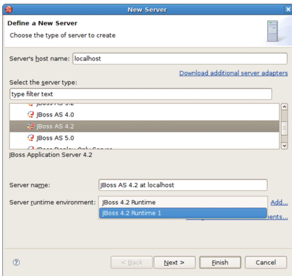
Figure 2.11. Choosing Runtime
