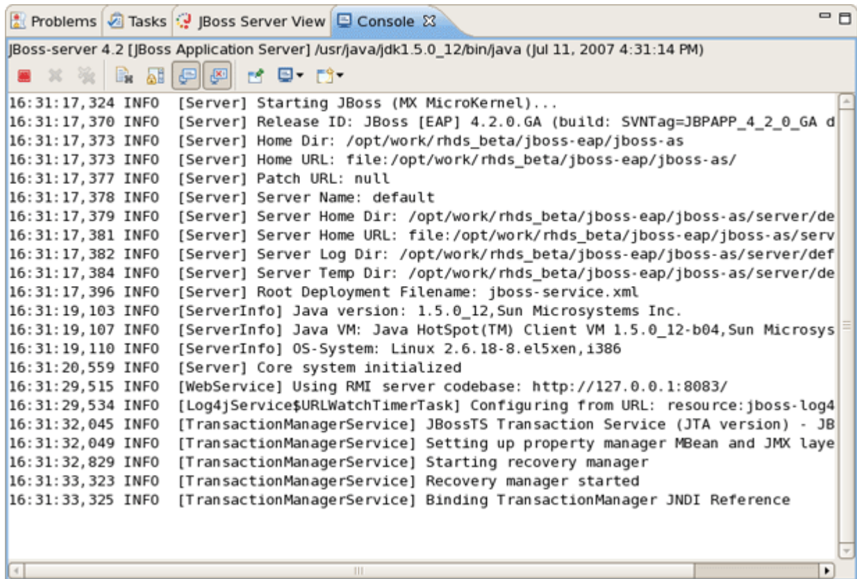
Figure 2.3. Console Output
