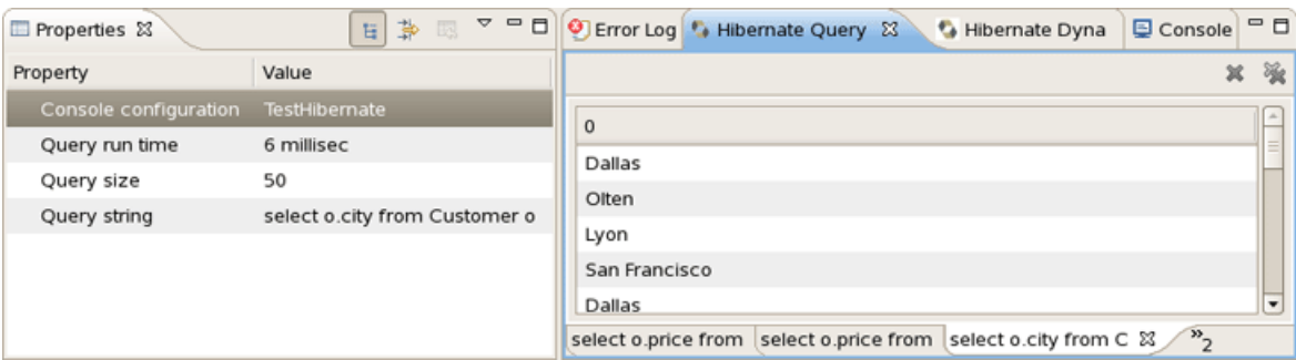
Figure 4.39. Properties View
