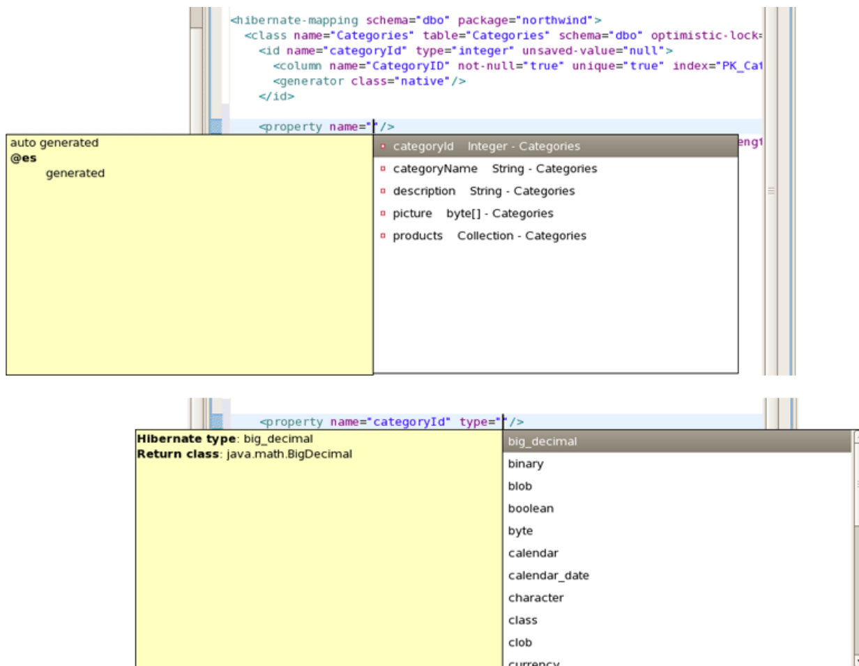
Figure 4.17. Navigation Functionality
