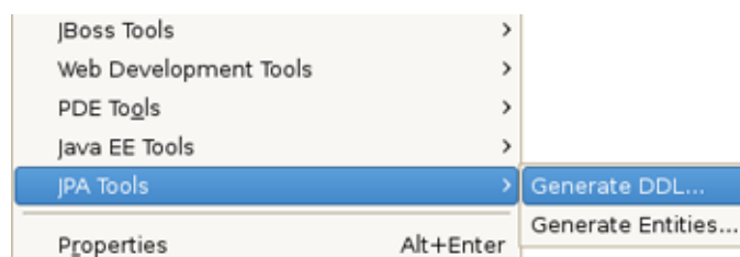
Figure 4.42. Generate DDL/Entities
