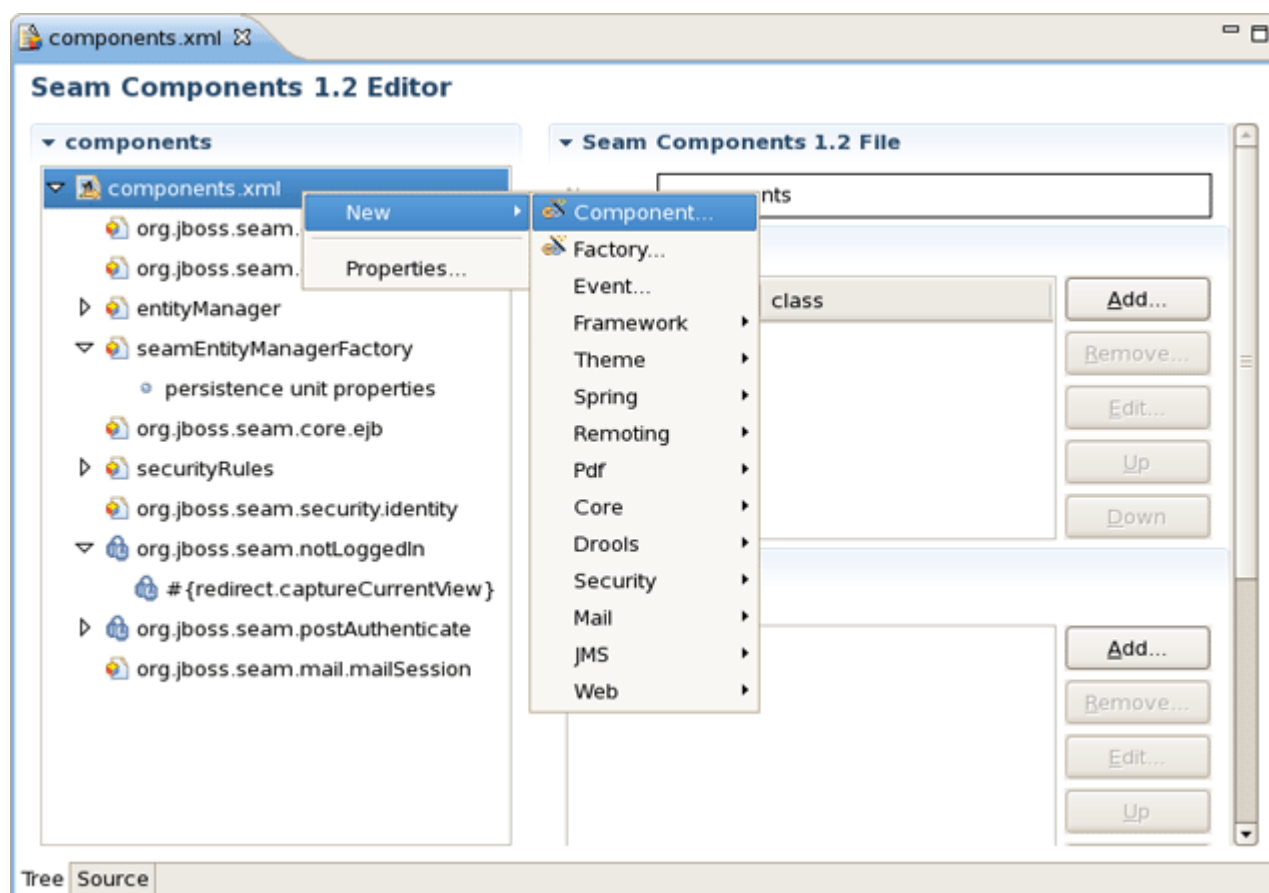
Figure 7.7. component.xml Editor
