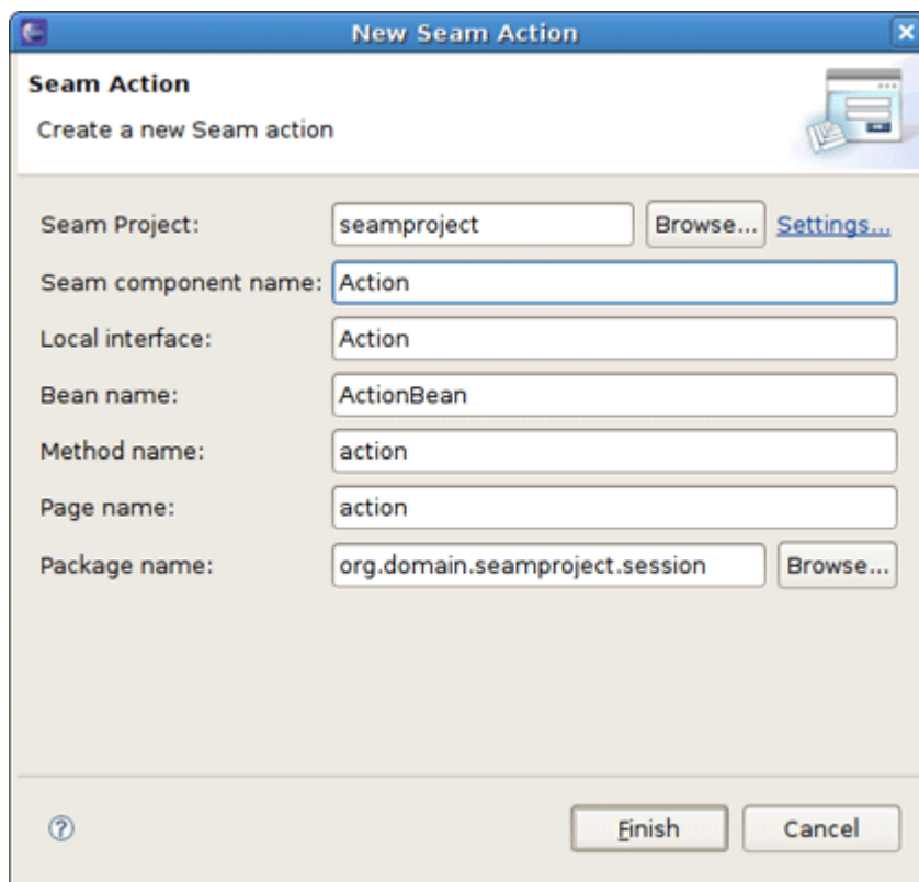
Figure 9.8. Settings Link
