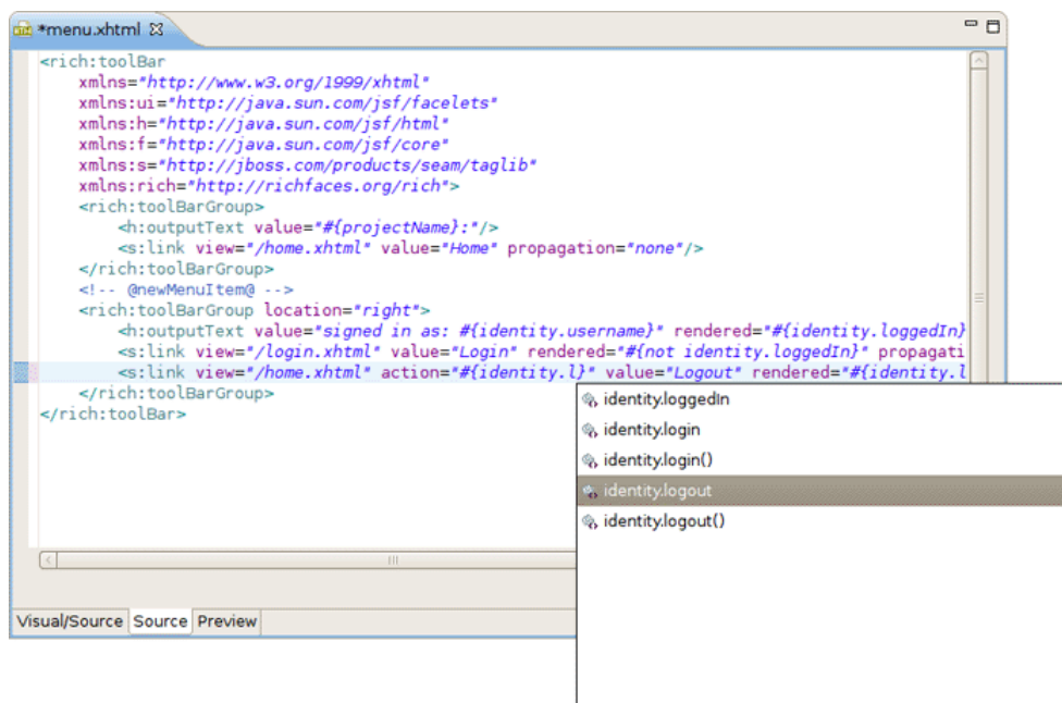
Figure 7.1. Content Assist
