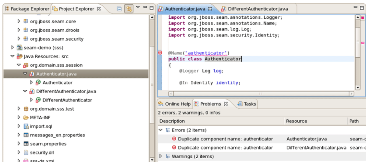
Figure 7.5. Seam Validation
