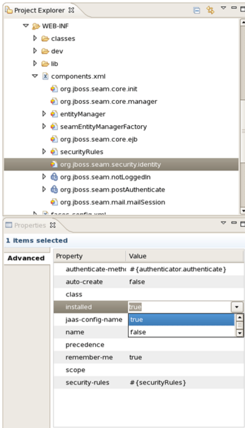
Figure 7.8. component.xml Editor
