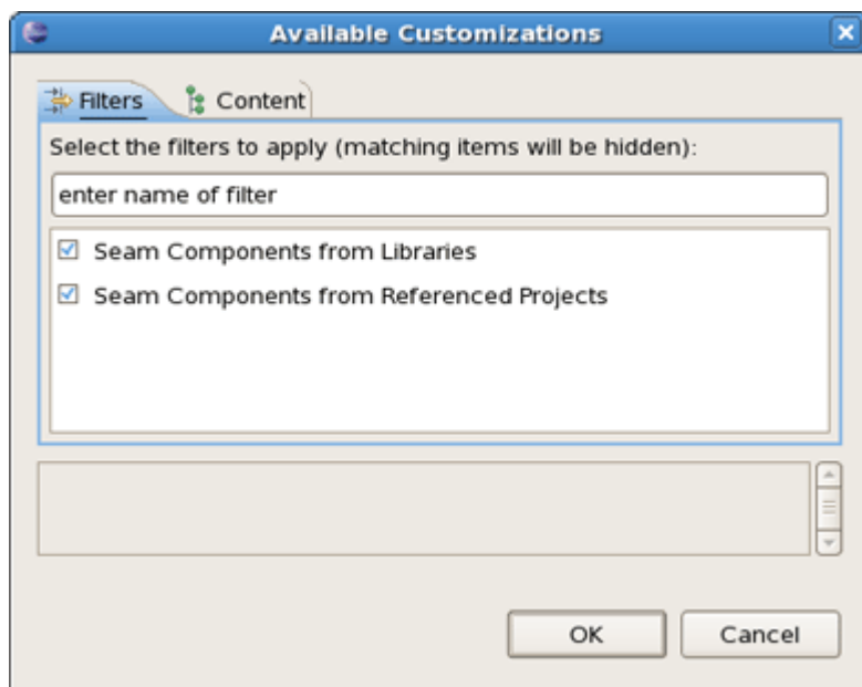
Figure 8.7. Available Customizations
