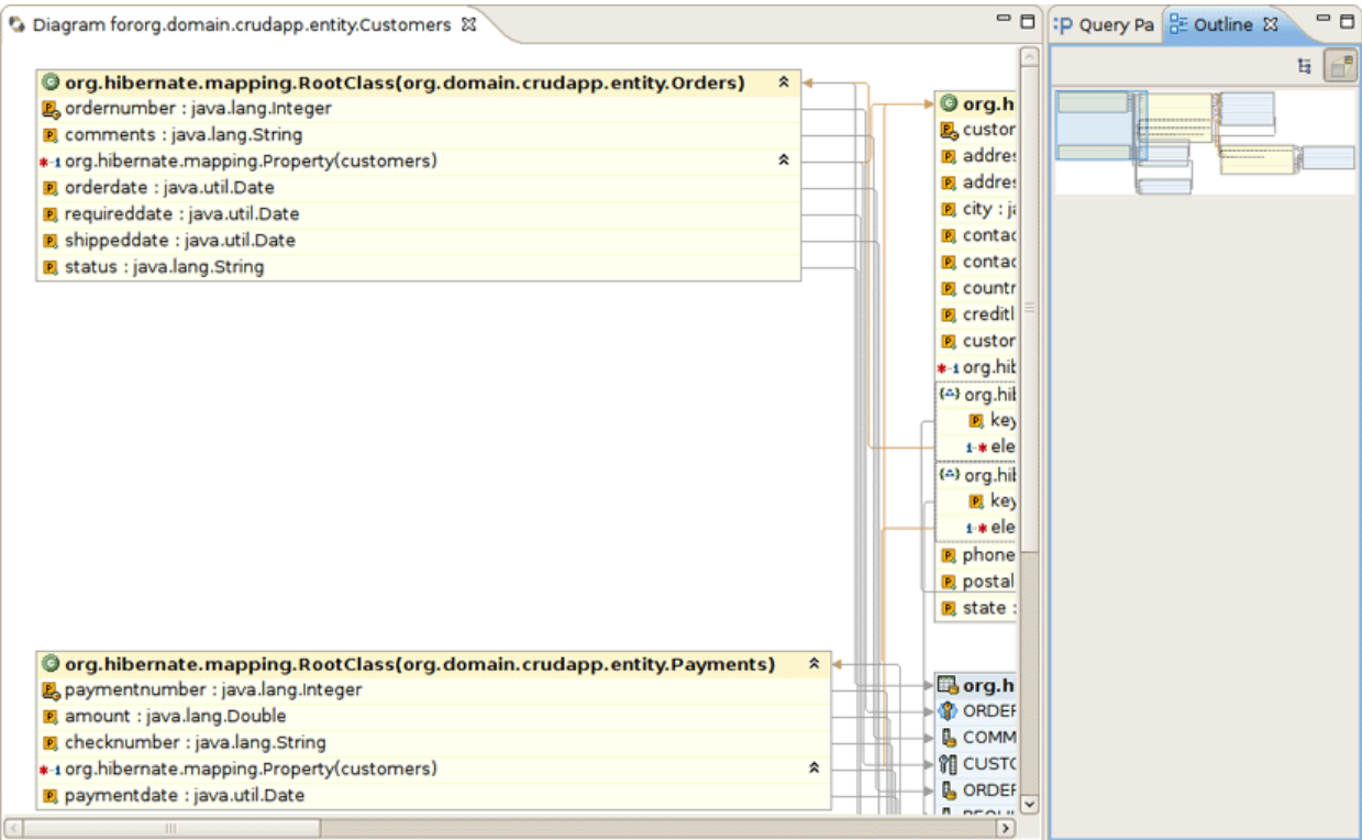
Figure 11.22. Mapping Diagram
