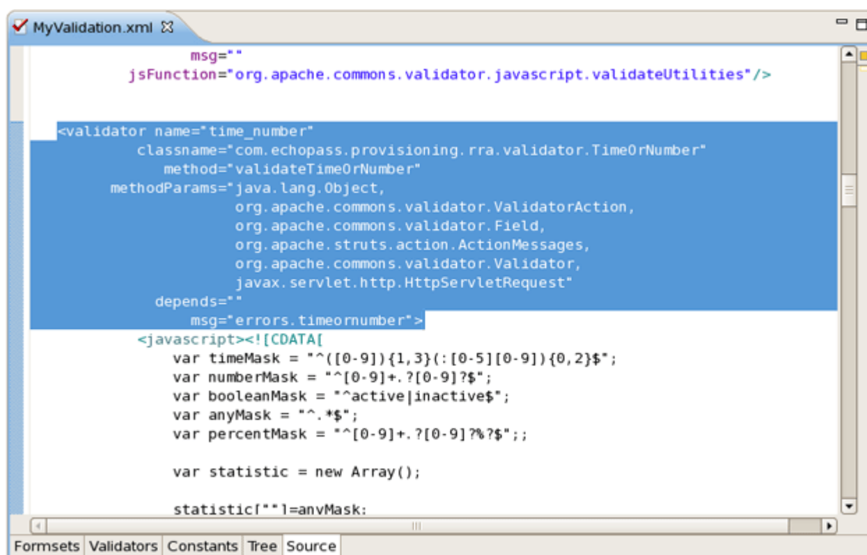
Figure 3.26. Validation Rules
