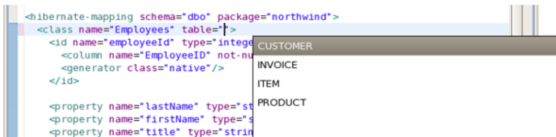
Figure 4.19. Table and Column Completion
