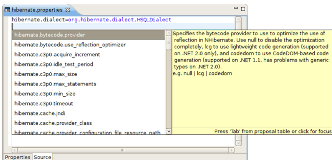
Figure 4.26. Content Assist in the Source view
