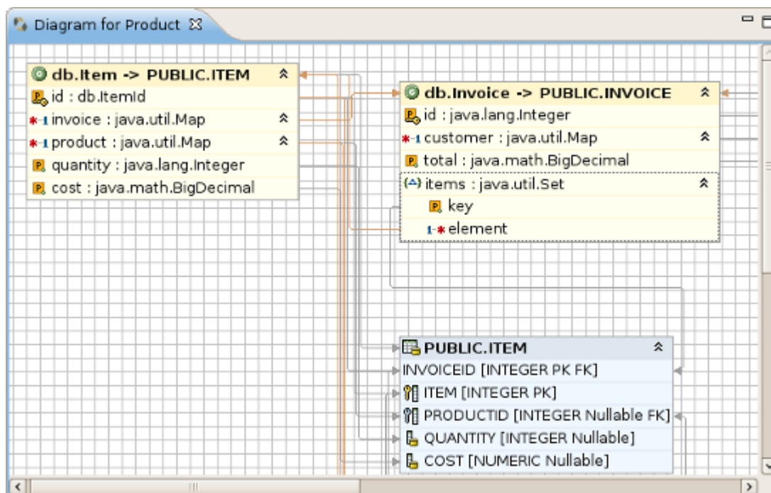
Figure 4.38. Grid on Mapping diagram
