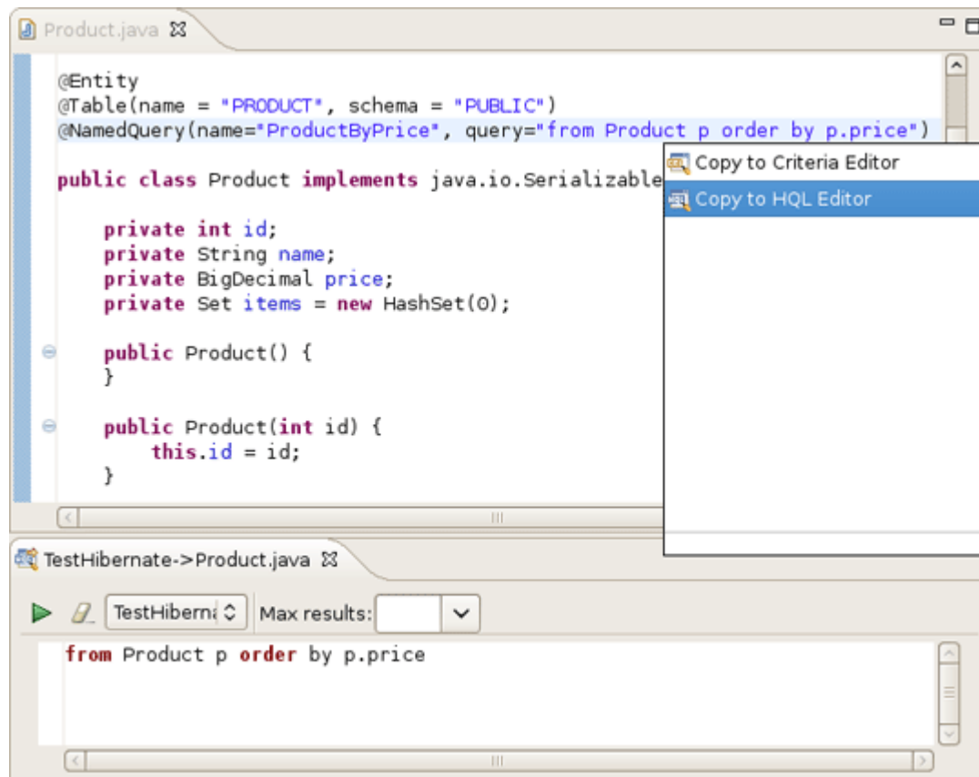
Figure 4.47. Quick Fix Option Demonstration
