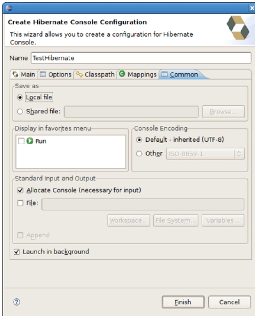
Figure 4.8. Common Tab of the Console Configuration Wizard
