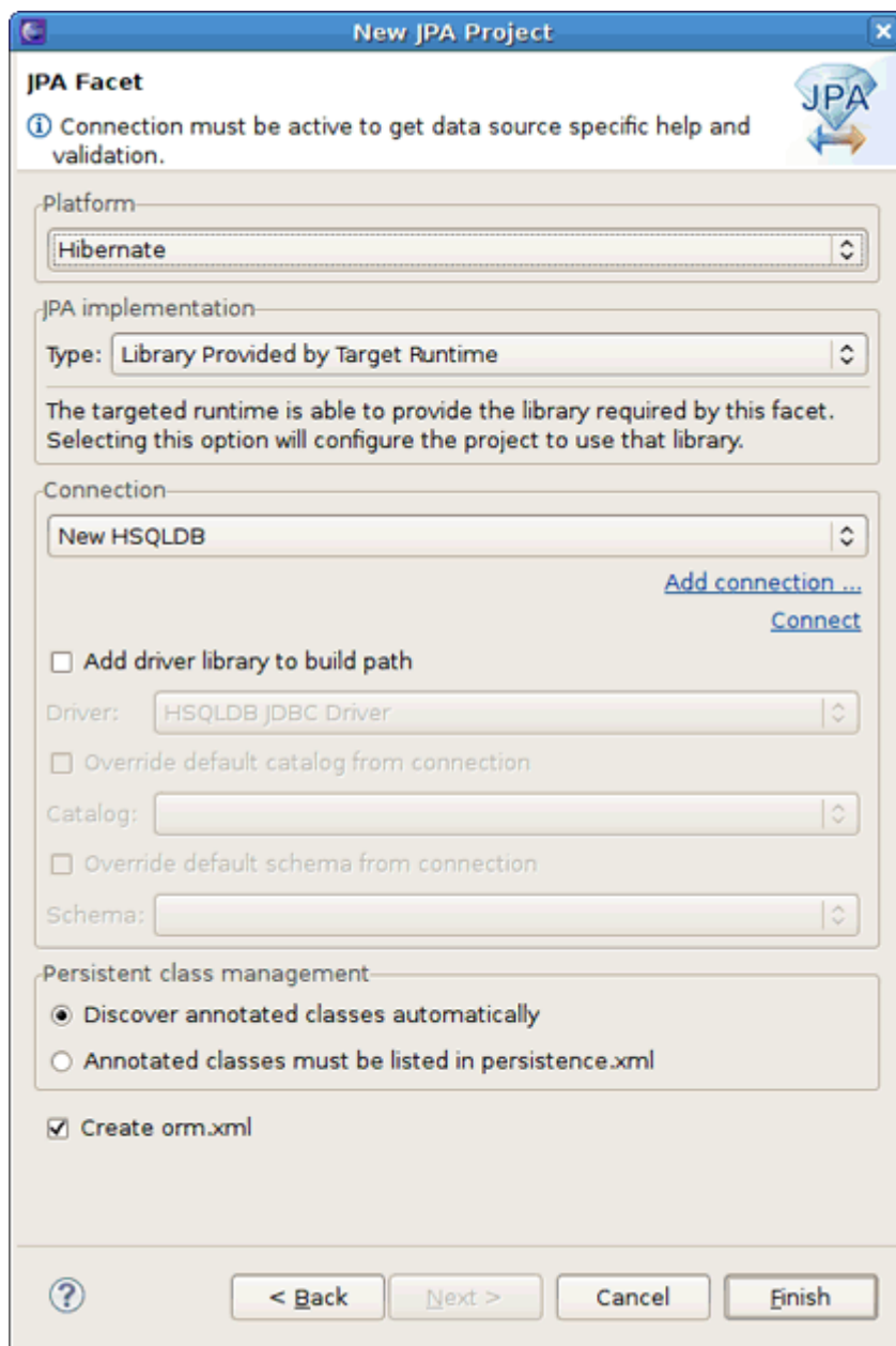
Figure 4.56. Targeting at Hibernate Platform
