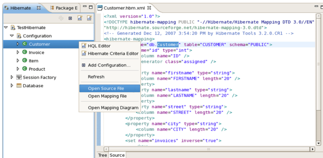
Figure 4.34. Opening Source for Objects
