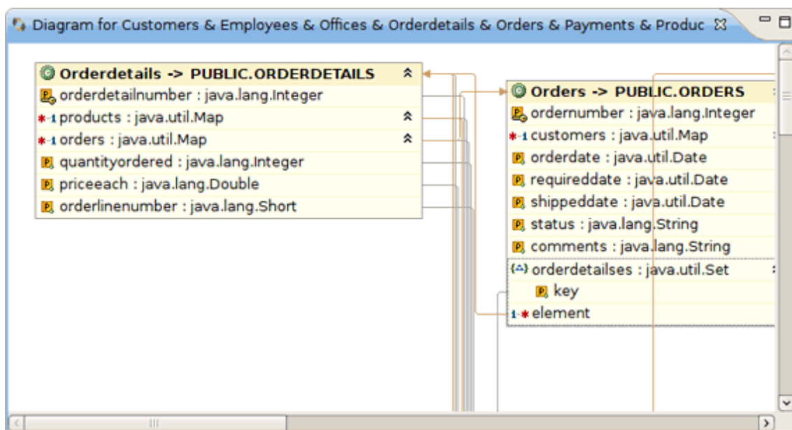
Figure 4.44. The Diagram after Refreshing
