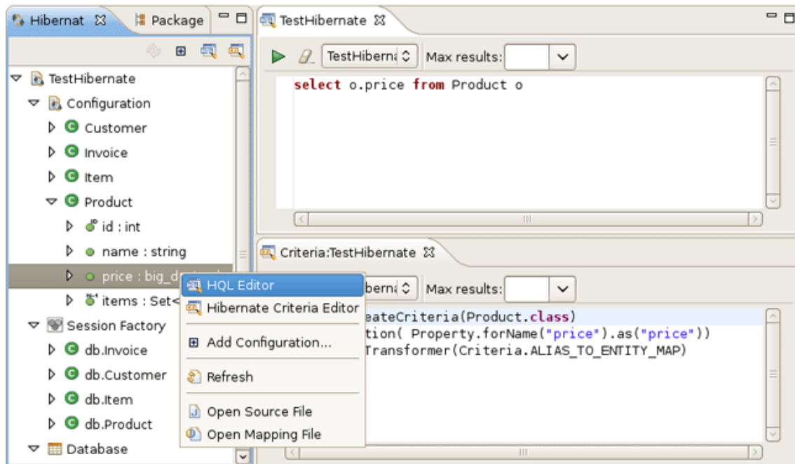
Figure 4.46. Generating Simple Queries
