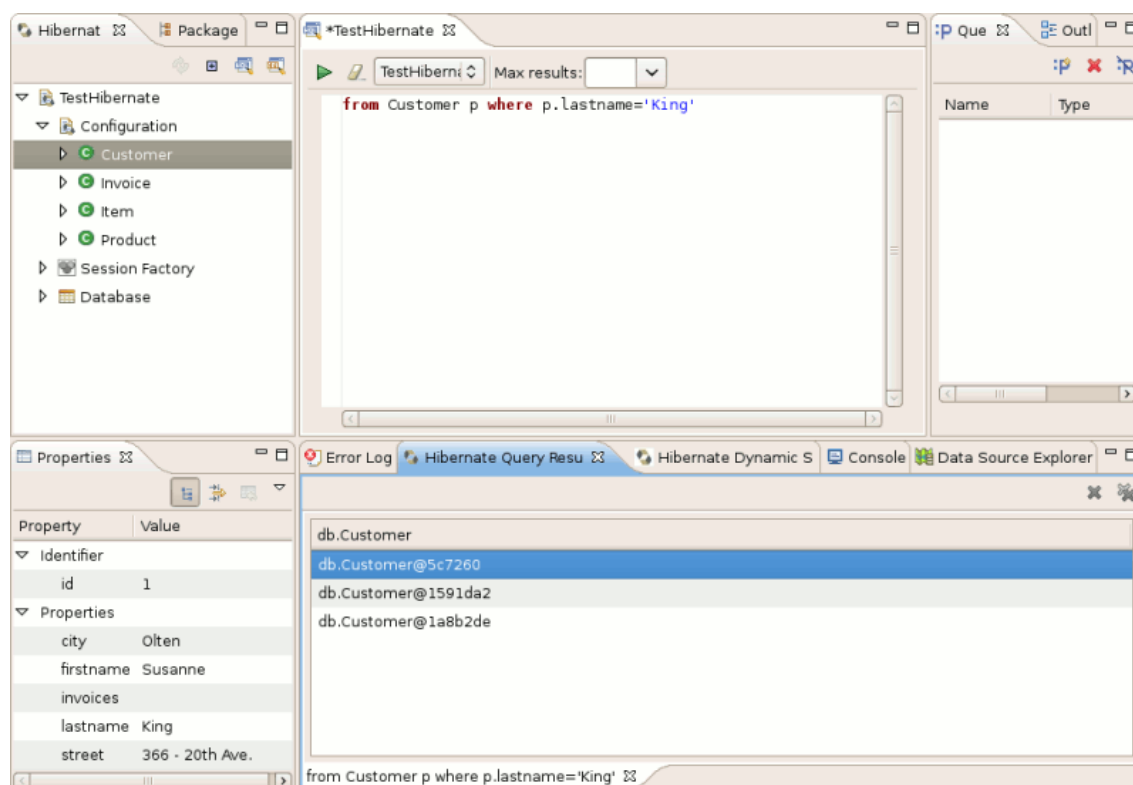
Figure 4.33. Hibernate Console Perspective
