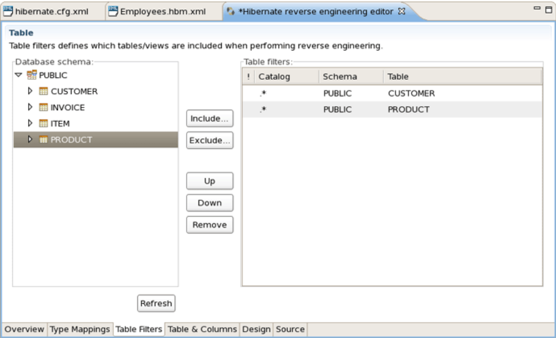
Figure 4.30. Table Filters Page
