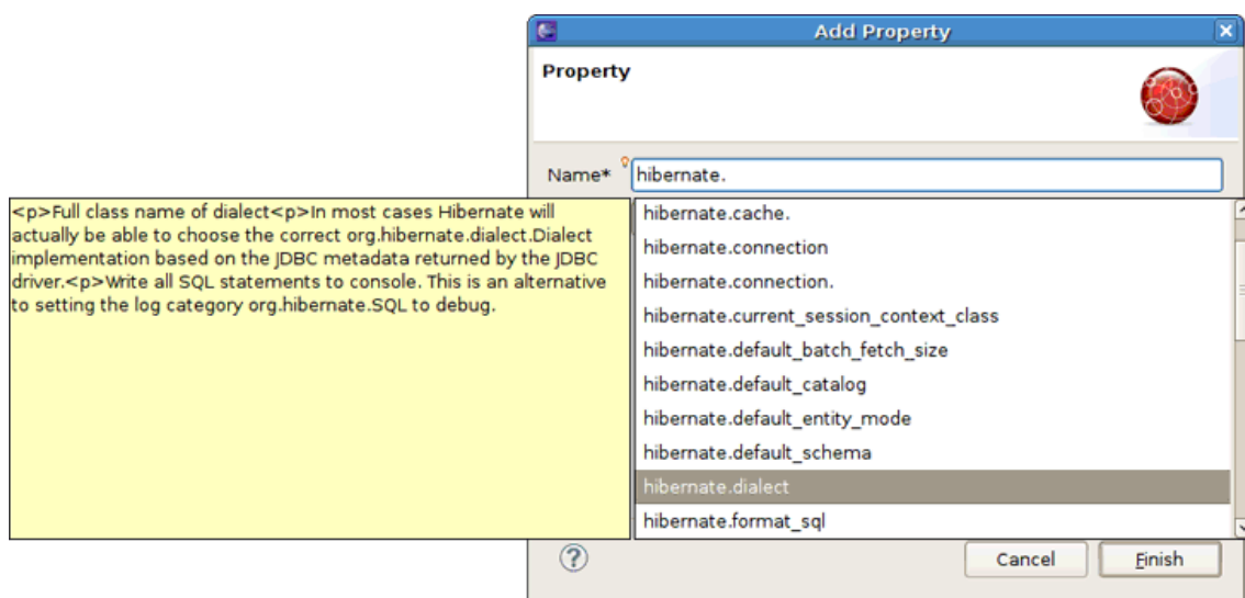
Figure 4.24. Content Assist for Properties Names
