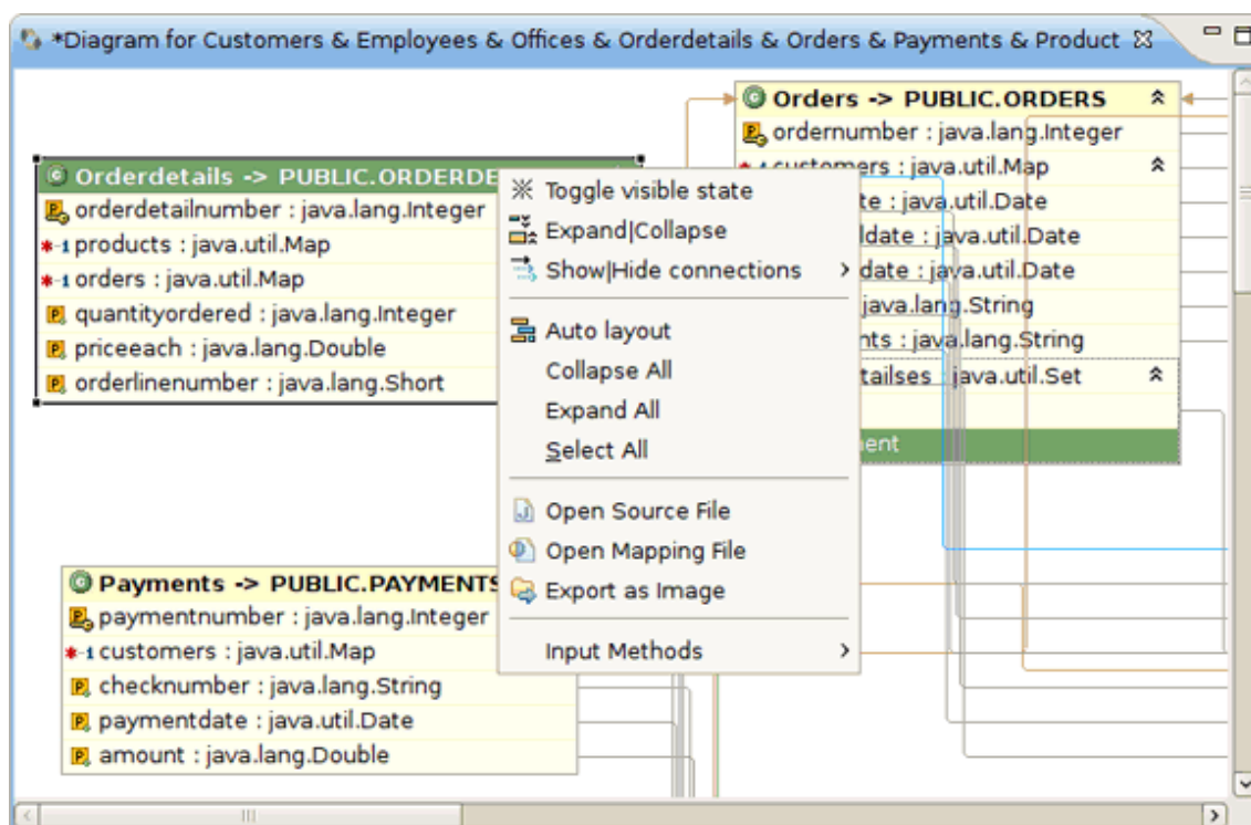
Figure 4.41. Context Menu in Mapping Item
