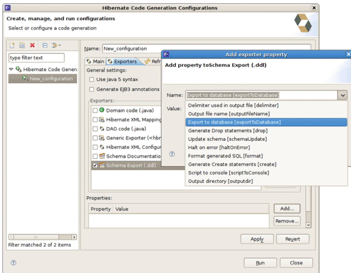
Figure 4.15. Adding the Property for Schema Export (.ddl)
