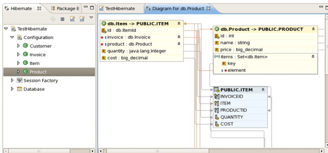
Figure 4.35. Mapping Diagram
