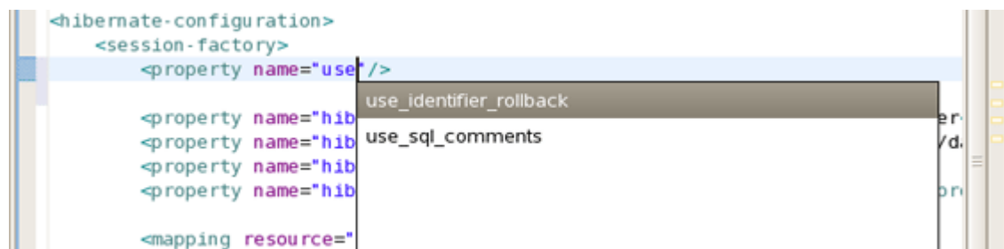
Figure 4.20. Property Completion
