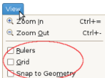
Figure 4.36. View menu
