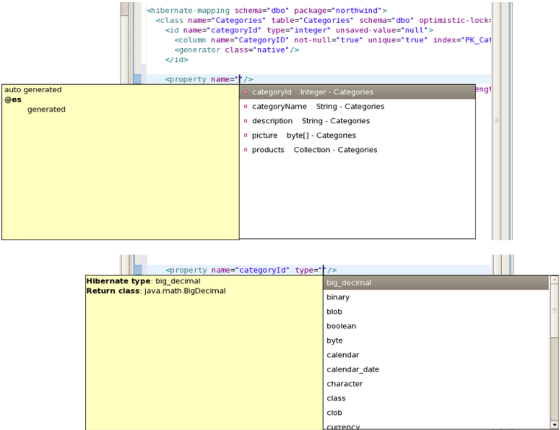
Figure 4.18. Navigation Functionality
