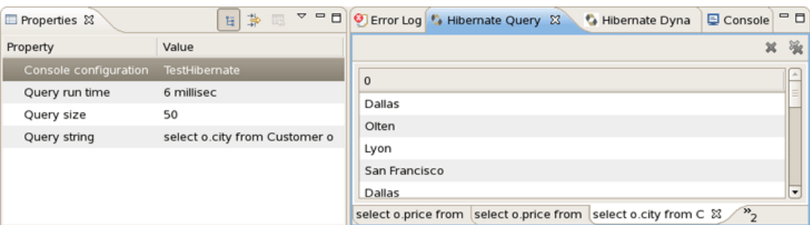
Figure 4.50. Properties View
