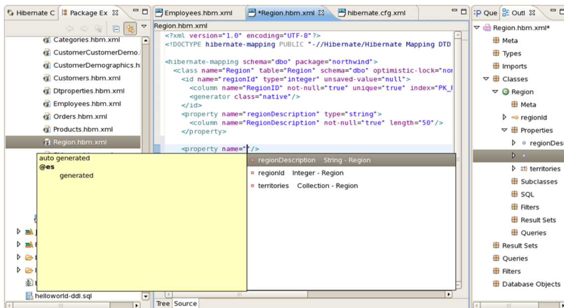
Figure 4.17. XML Editing Functionality
