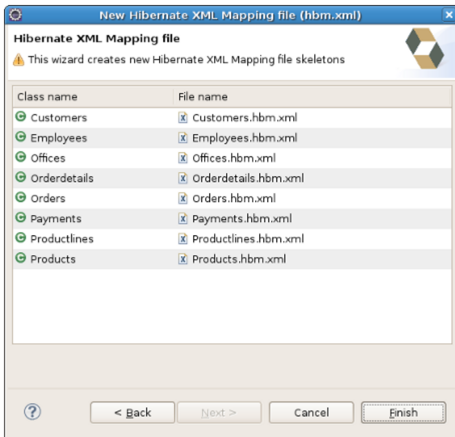
Figure 4.2. Mappings to be generated
