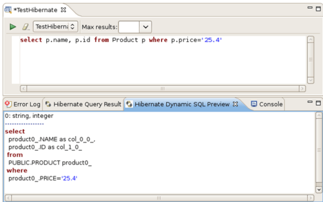
Figure 4.49. Hibernate Dynamic Query Translator View
