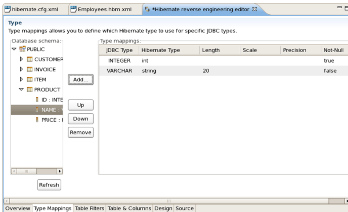
Figure 4.31. Type Mappings Page
