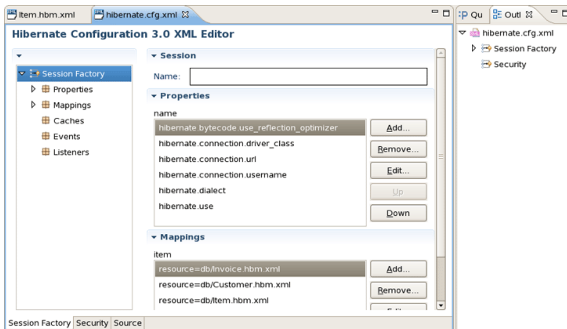
Figure 4.22. Structured cfg.xml Editor
