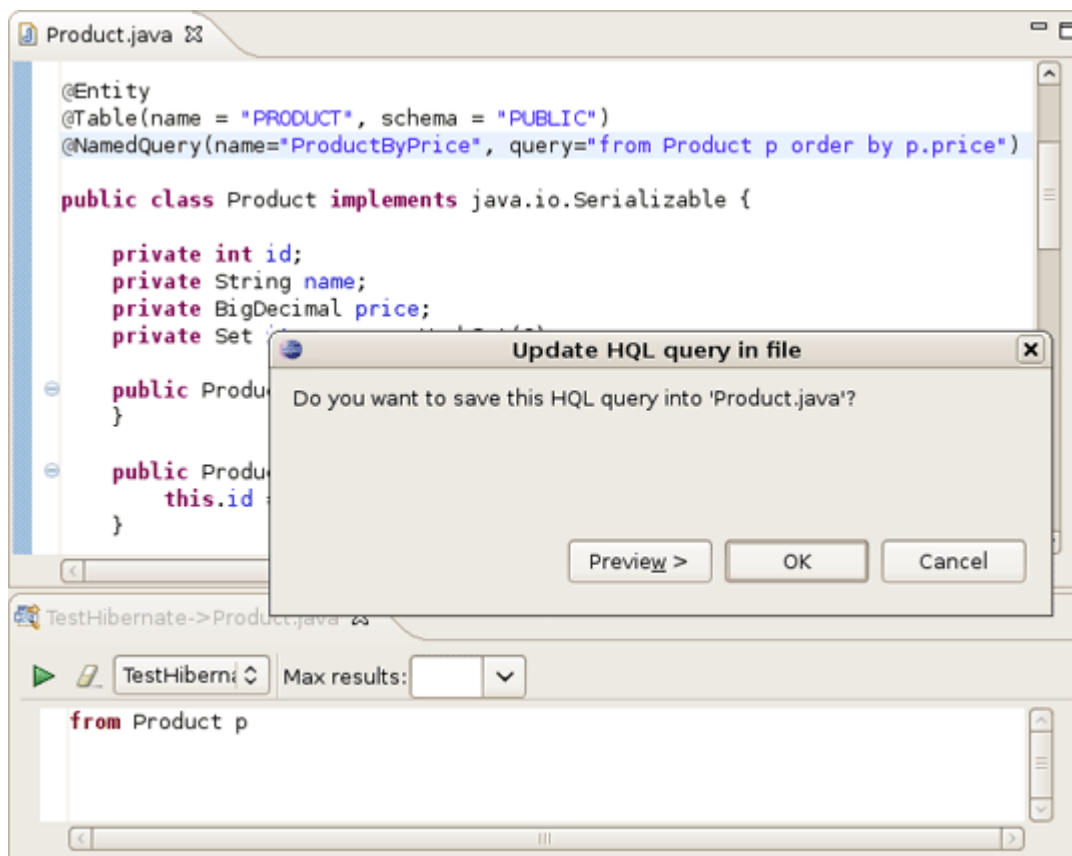
Figure 4.48. Updating Java Code
