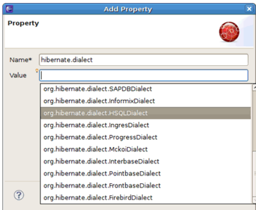
Figure 4.25. Content Assist for Properties Values
