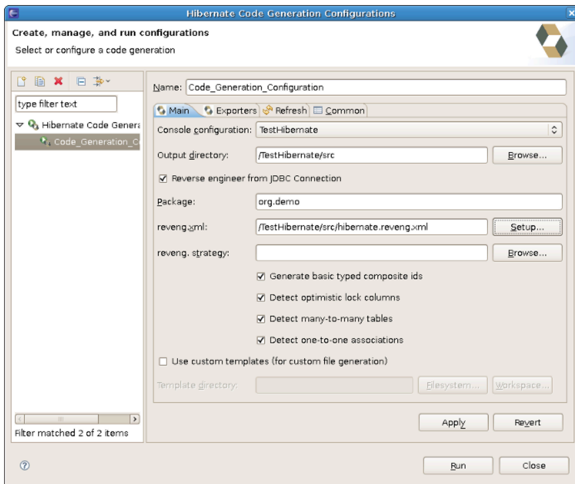
Figure 4.13. Hibernate Code Generation Wizard
