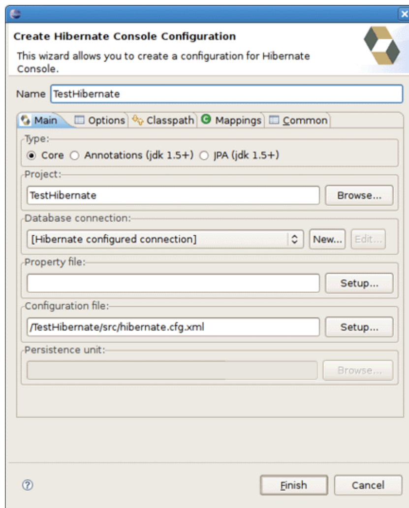
Figure 4.4. Creating Hibernate Console Configuration
