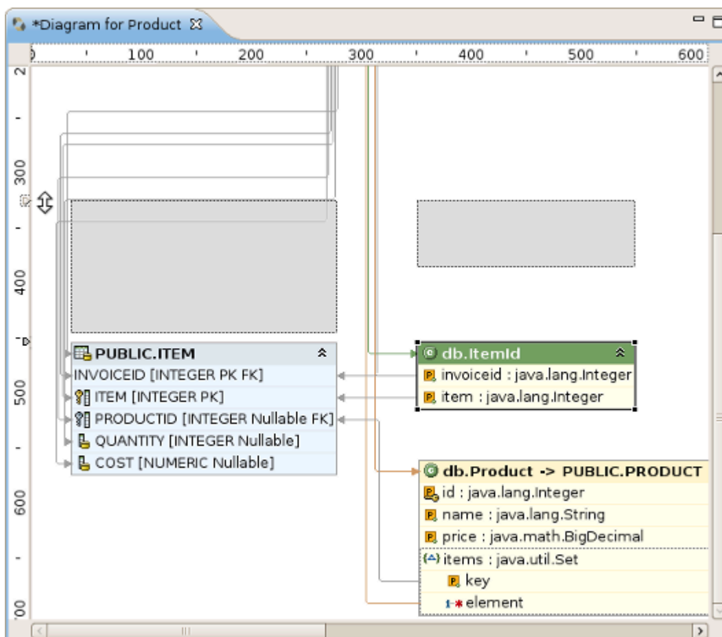
Figure 4.37. Moving the Ruler guide
