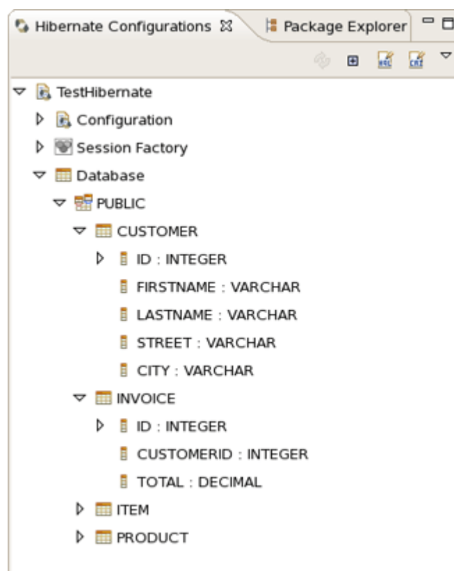
Figure 4.9. Console Overview
