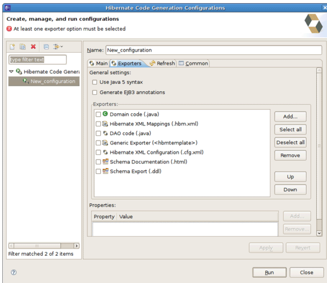
Figure 4.14. Selecting Exporters
