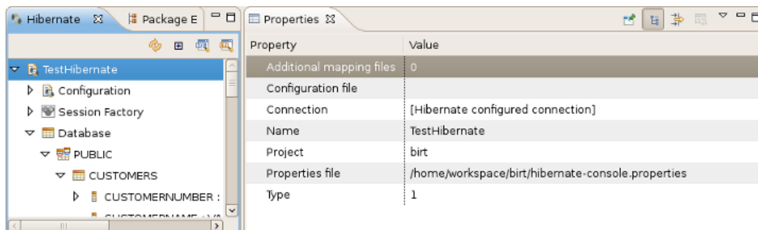
Figure 4.11. Properties View
