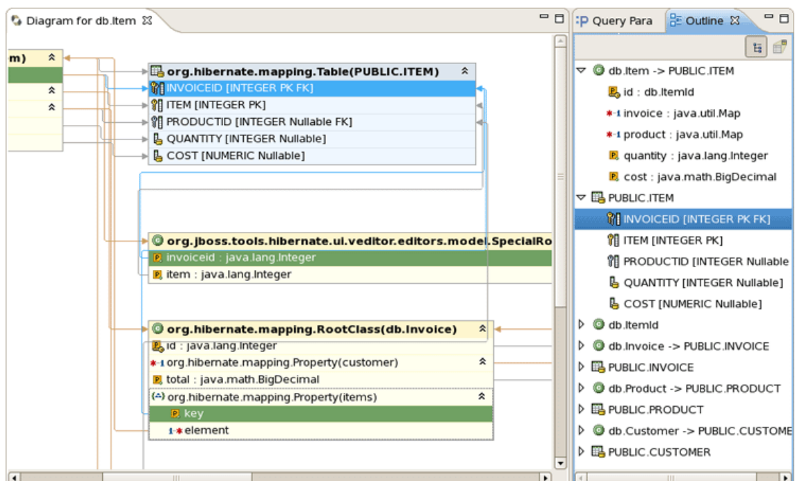
Figure 4.39. Navigating in the Structural Mode
