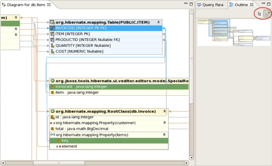
Figure 4.40. Navigating in the Graphical Mode
