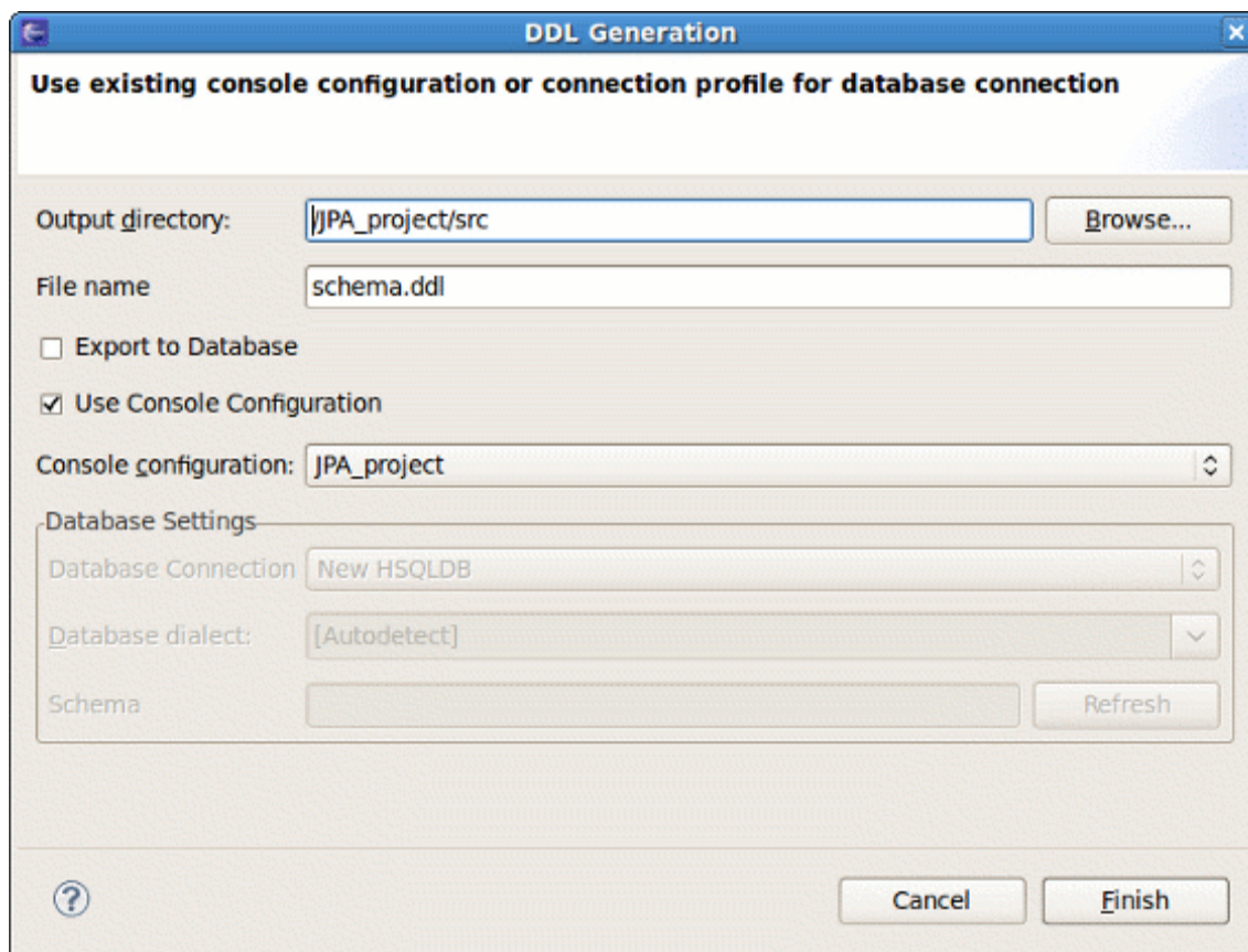
Figure 4.60. Generate DDL Wizard
