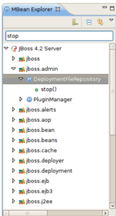
Figure 2.2. Query Filter
