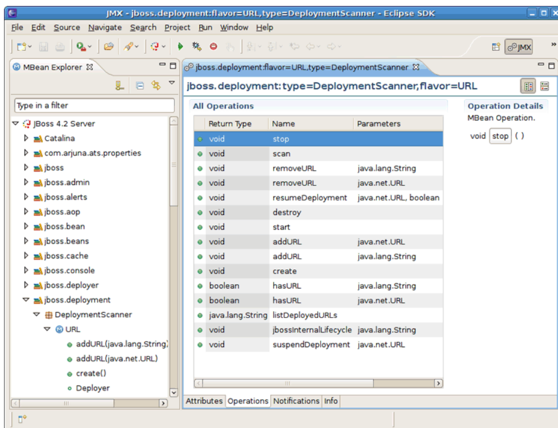
Figure 1.1. JMX Tools
