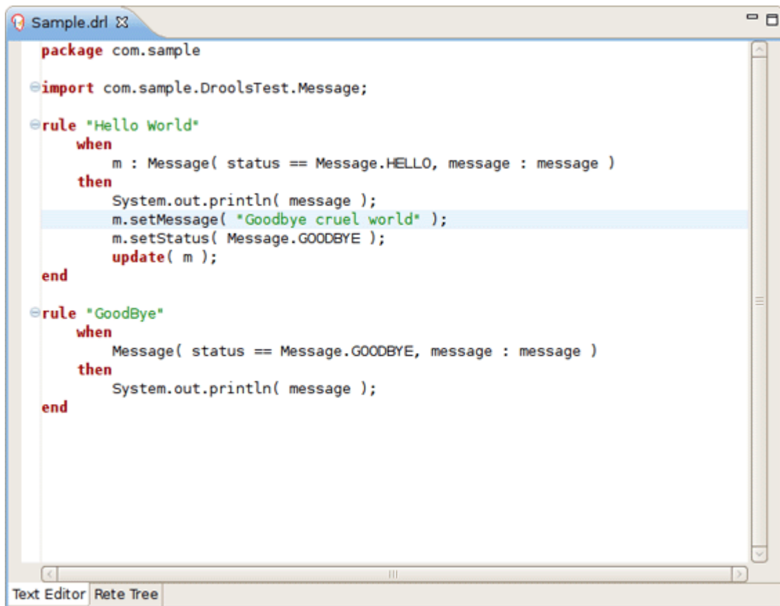
Figure 4.9. New Rule
