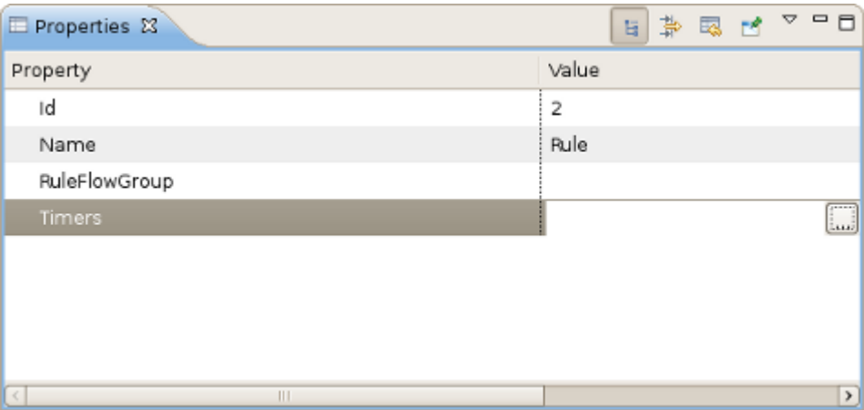
Figure 4.7. Properties view
