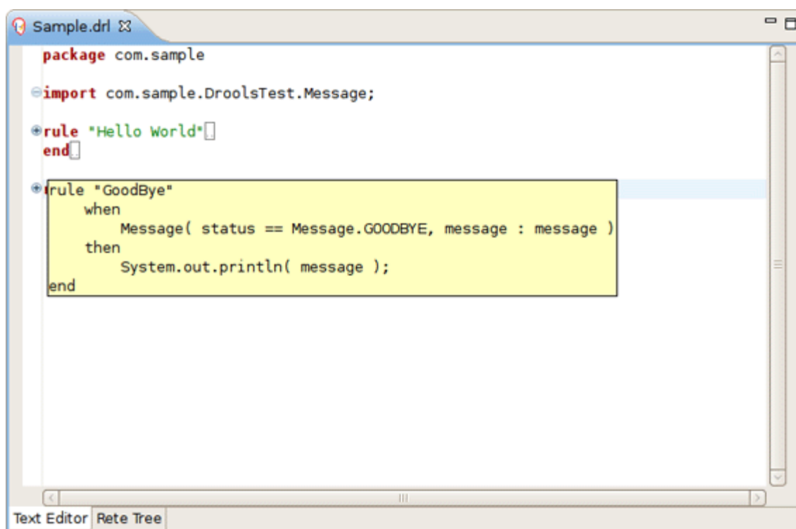
Figure 4.12. Code Folding
