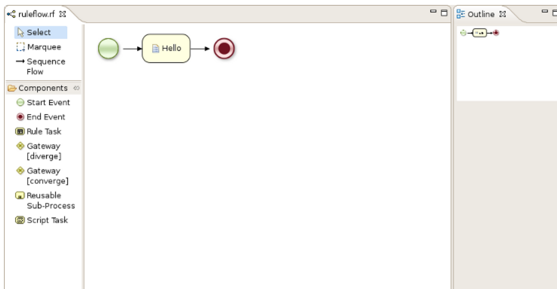
Figure 4.5. Flow Editor
