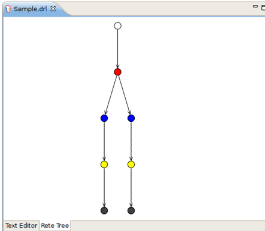
Figure 4.14. Rete Tree
