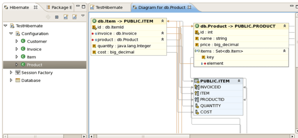
Figure 4.37. Mapping Diagram
