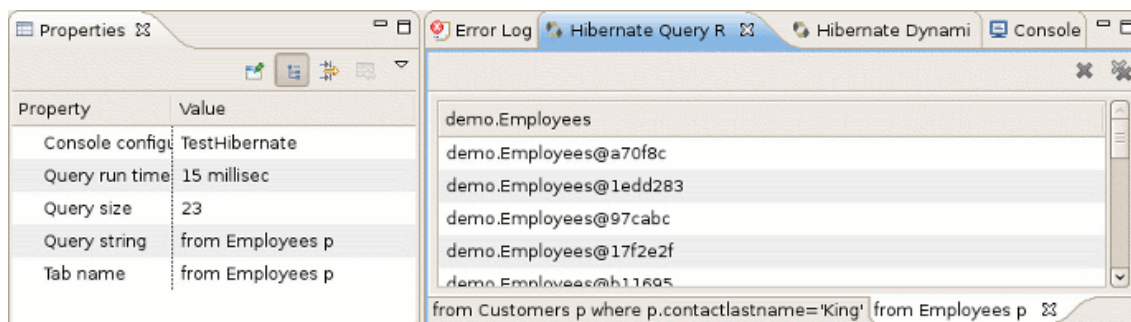
Figure 4.54. Properties View
