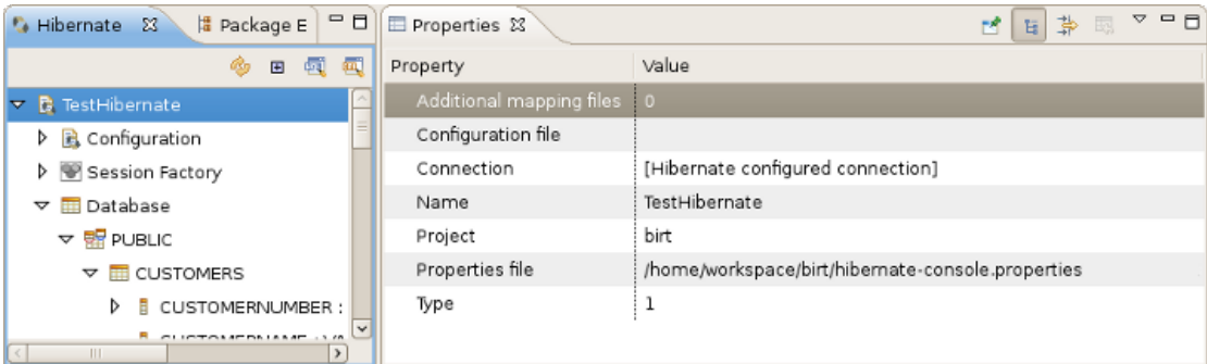
Figure 4.12. Properties View
