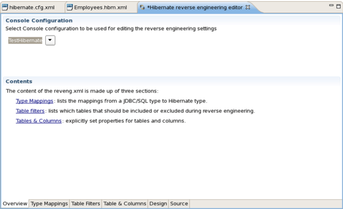
Figure 4.31. Overview Page
