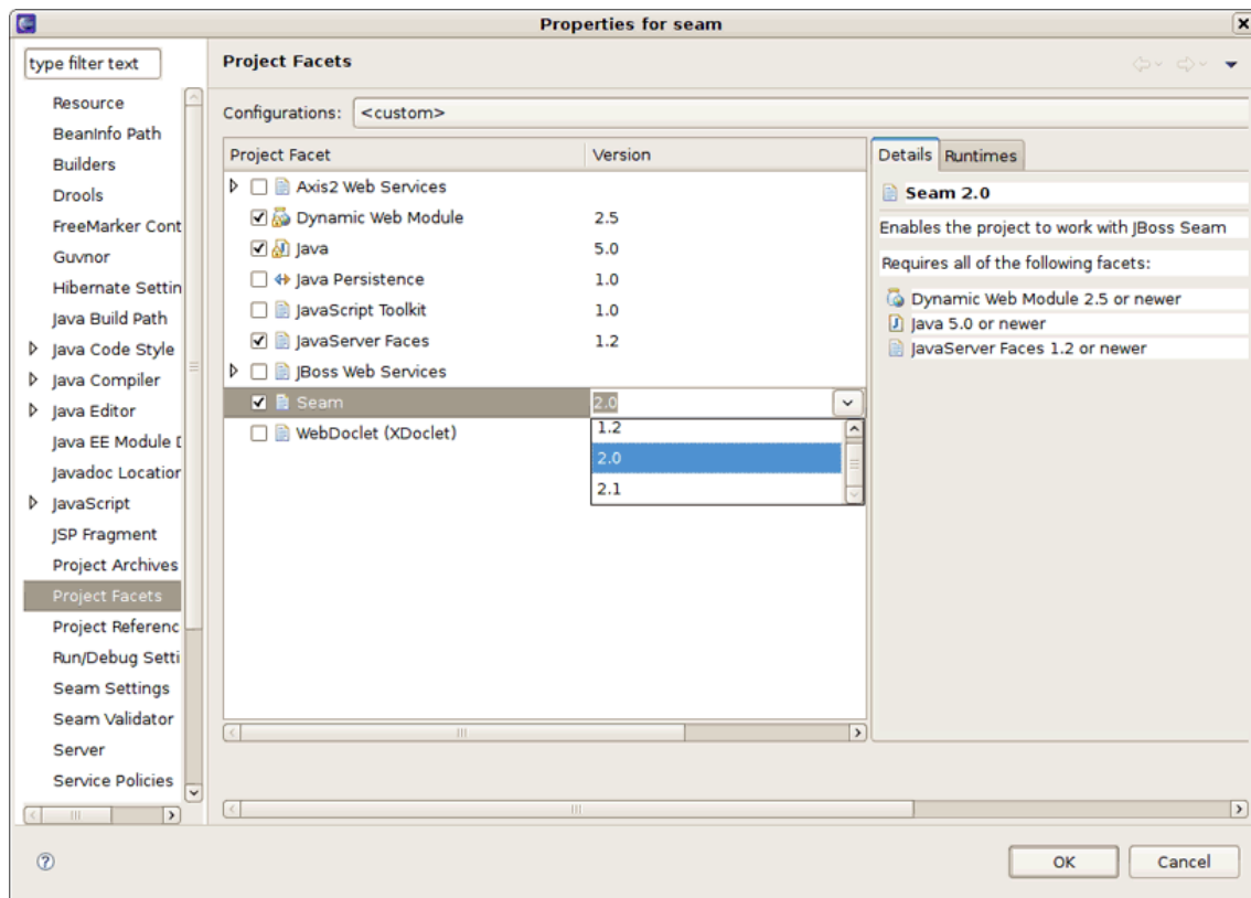
Figure 4.3. Changing the Seam Facet Version
