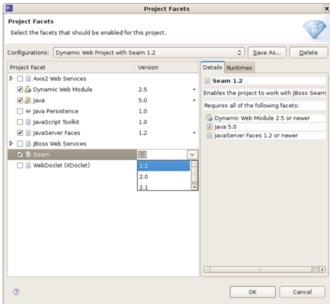
Figure 2.10. Project Facets Selection
