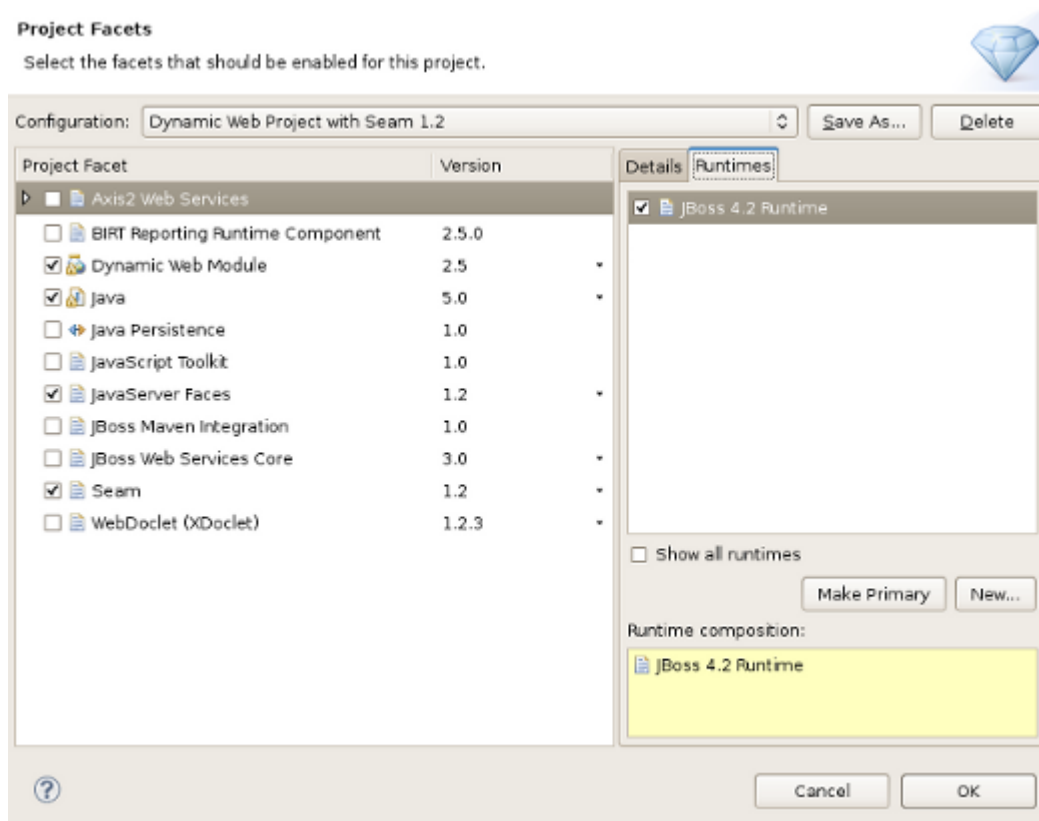
Figure 2.12. Setting Runtime
