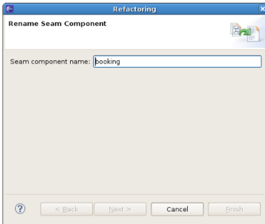
Figure 11.2. Refactoring Wizard
