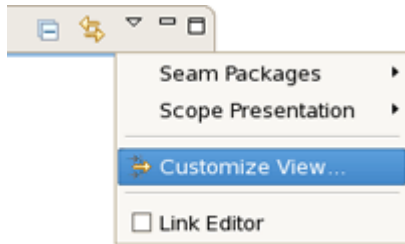
Figure 9.6. Customize View
