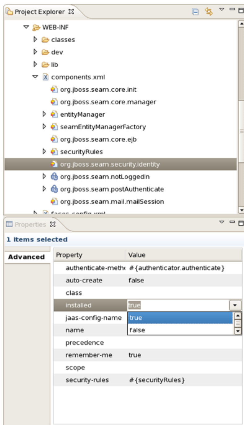
Figure 8.7. component.xml Editor
