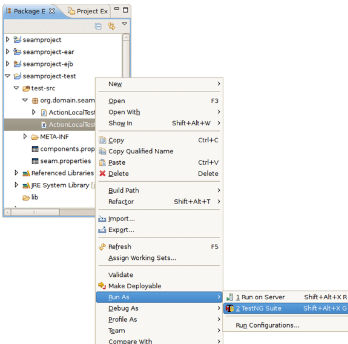
Figure 15.5. Running TestNG
