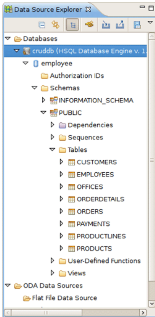
Figure 13.15. CRUDB Database
