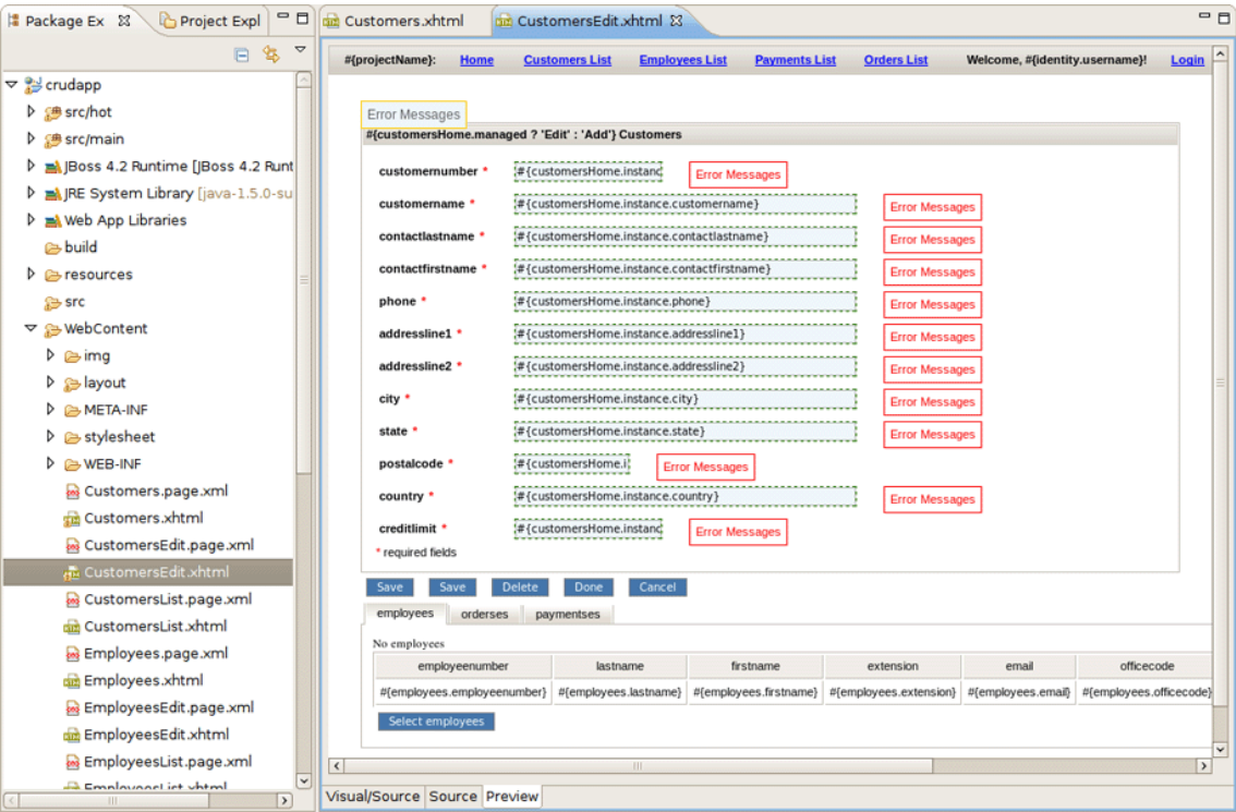
Figure 13.19. Entities Web Pages
