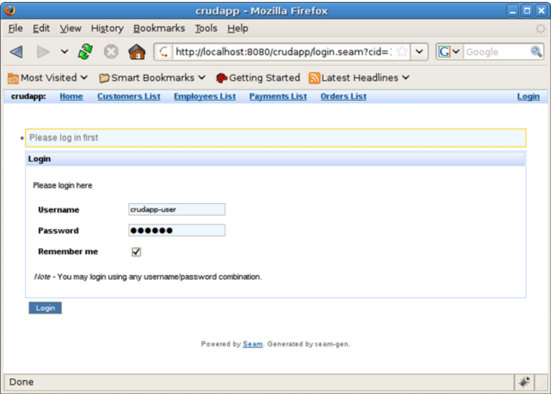
Figure 14.6. Login page
