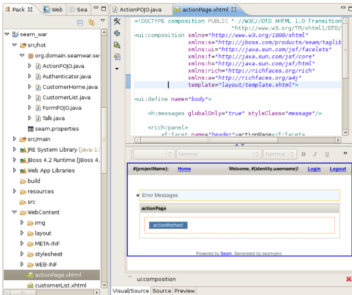
Figure 6.5. Action Page in JBoss Tools HTML Editor.
