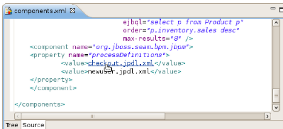
Figure 8.15. OpenOn in components.xml file
