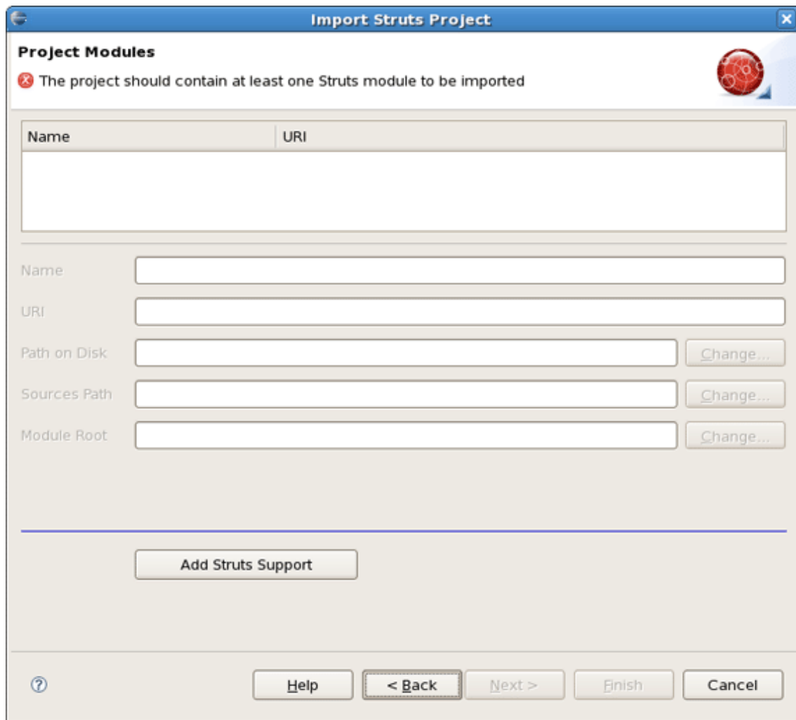
Figure 2.9. Project Modules
