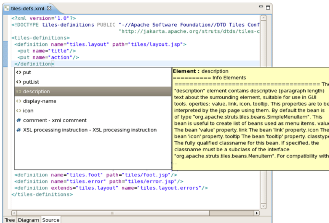
Figure 3.17. Code Assist
