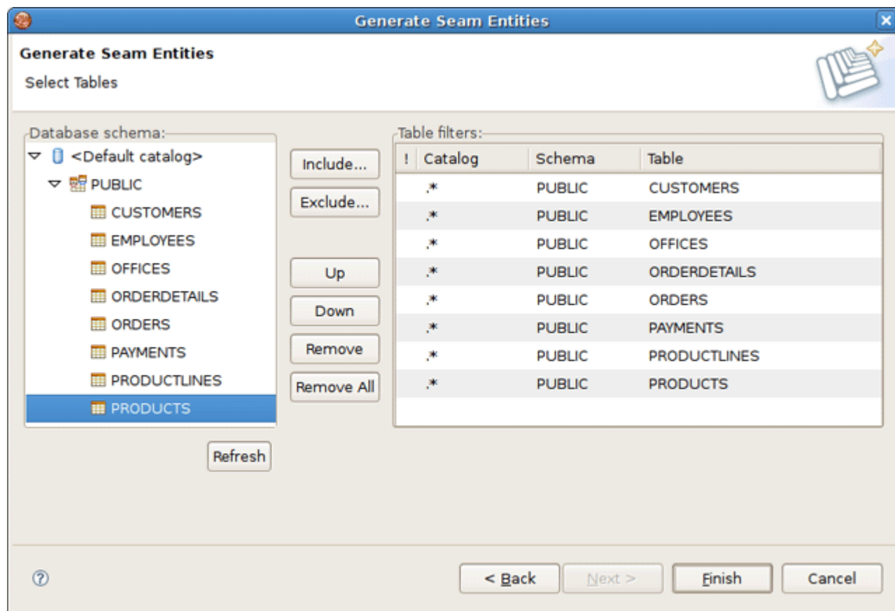
Figure 3.35. Selecting Tables
