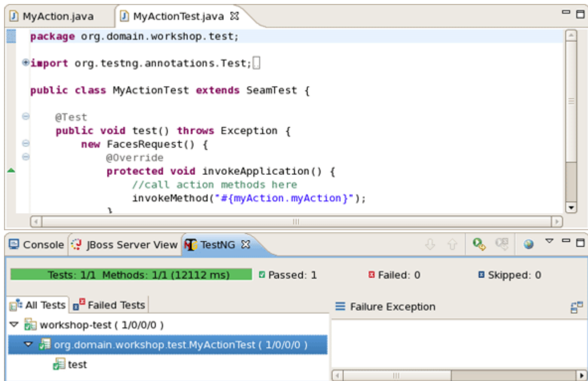
Figure 3.22. TestNG Results
