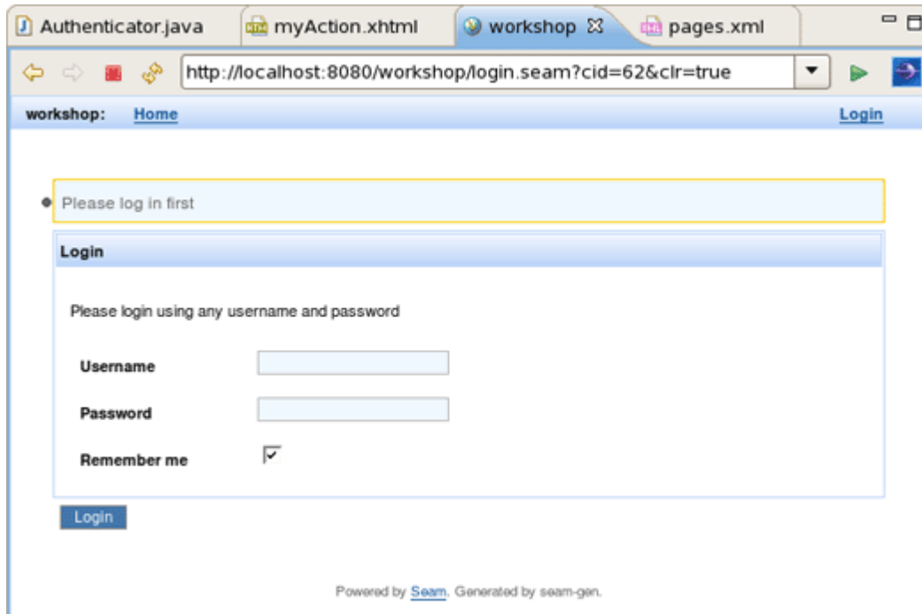
Figure 3.30. Login Page
