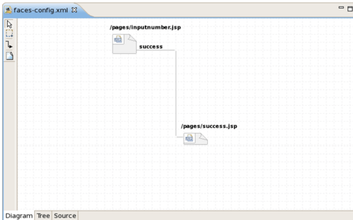
Figure 5.6. Created Connection
