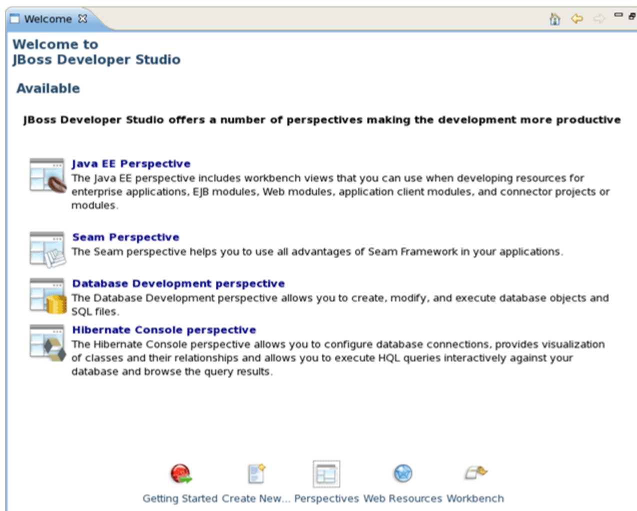
Figure 1.13. Perspectives
