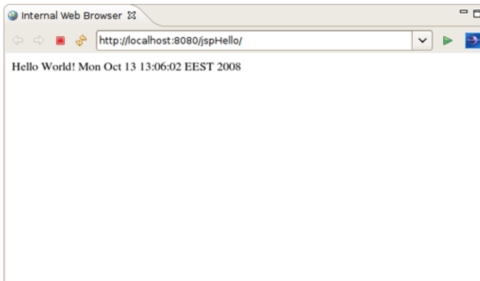
Figure 4.14. Running Project
