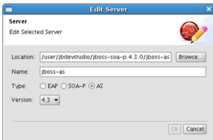
Figure 1.8. Edit Server
