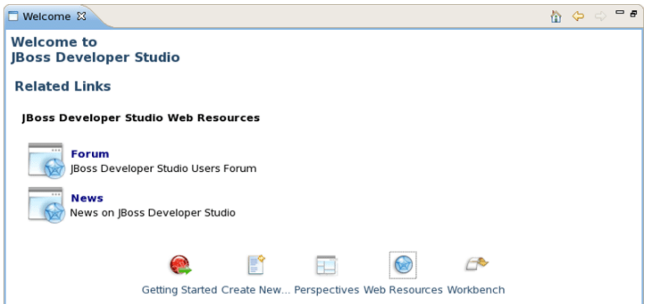
Figure 1.14. Web Resources
