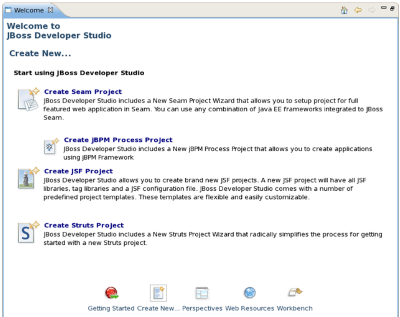
Figure 1.12. Create New...
