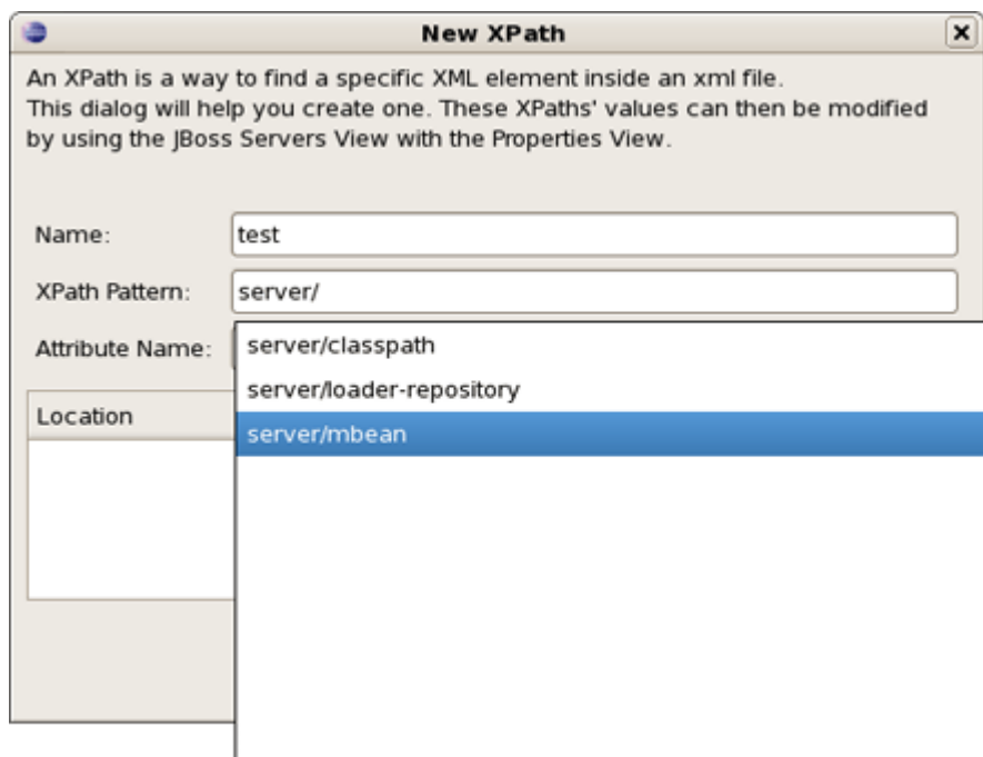
Figure 3.14. XPath Preview
