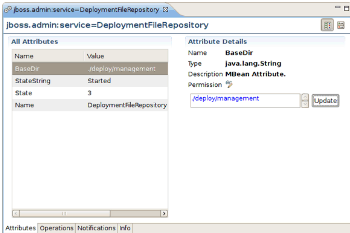
Figure 3.1. MBean Editor Pages
