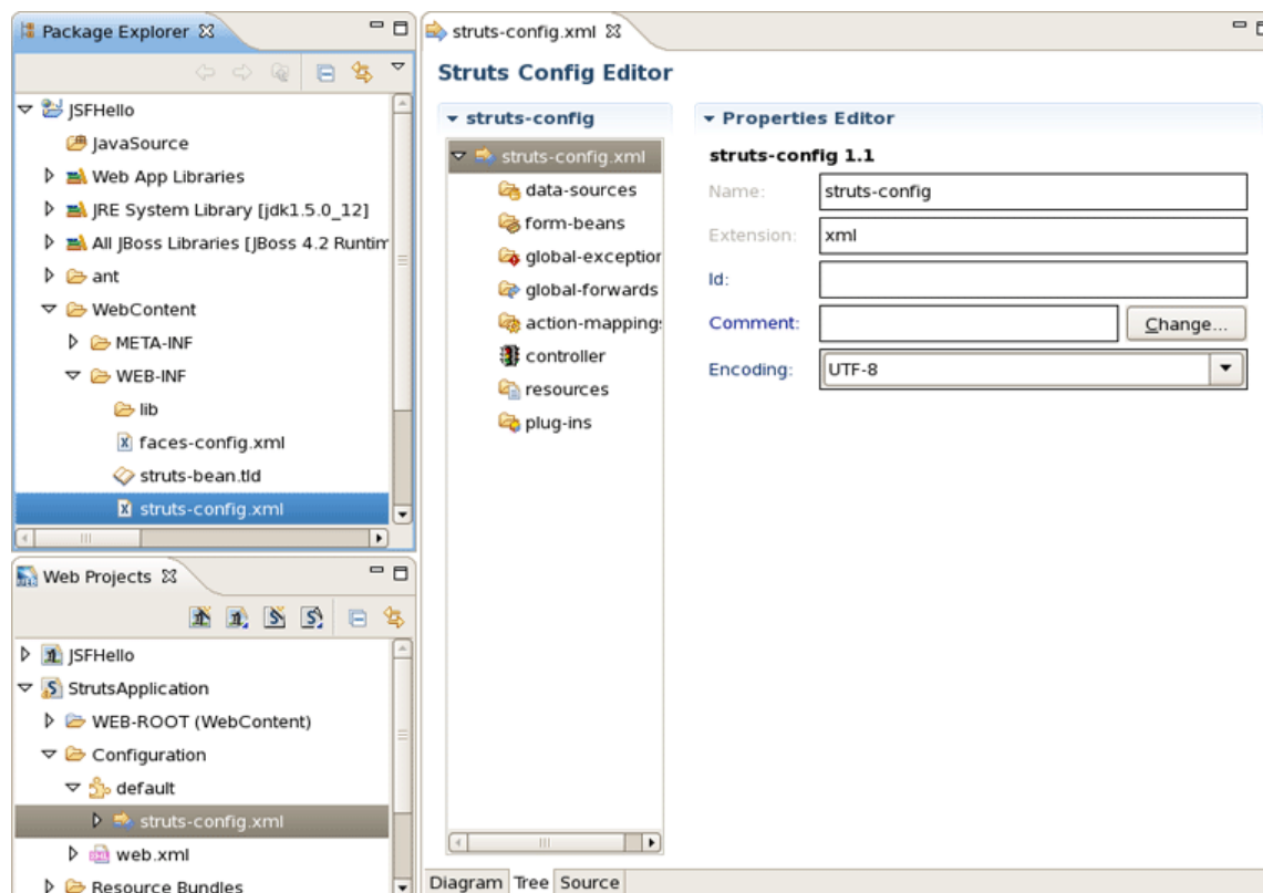
Figure 2.13. Struts-config.xml File
