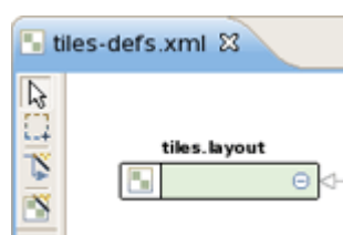
Figure 3.15. Diagram Toolbar
