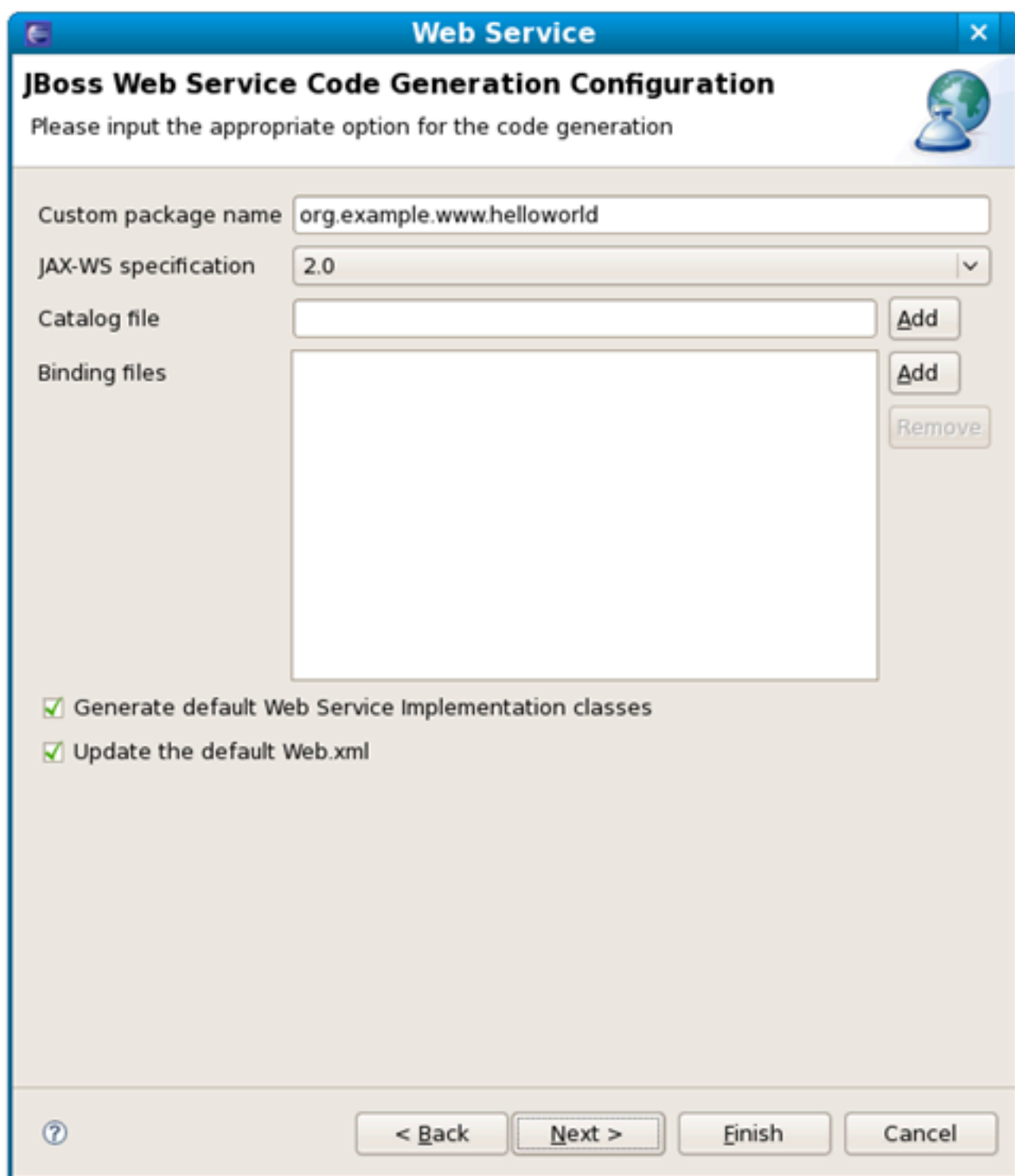
Figure 2.9. New Web Service Wizard
