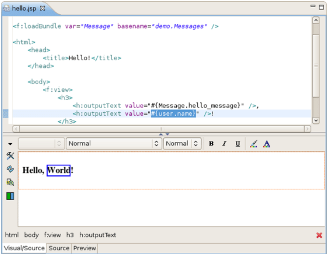
Figure 3.65. The EL Expression Value
