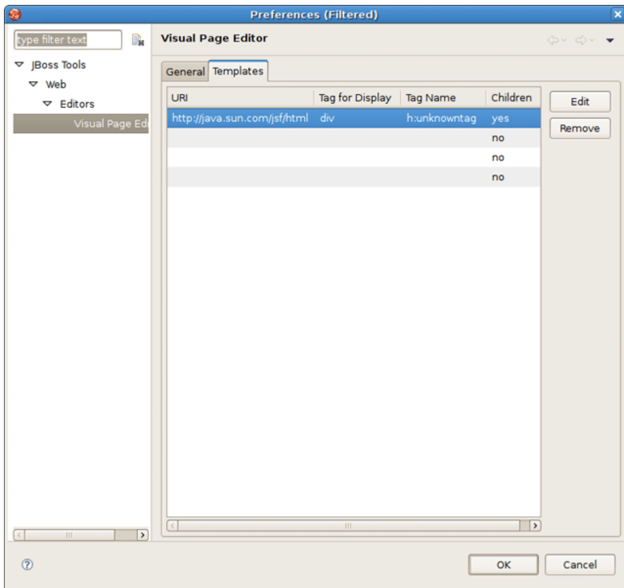
Figure 3.56. Templates Tab of the VPE Preferences Page
