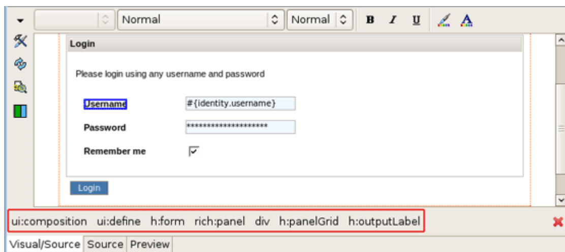
Figure 3.68. Selection Tag Bar
