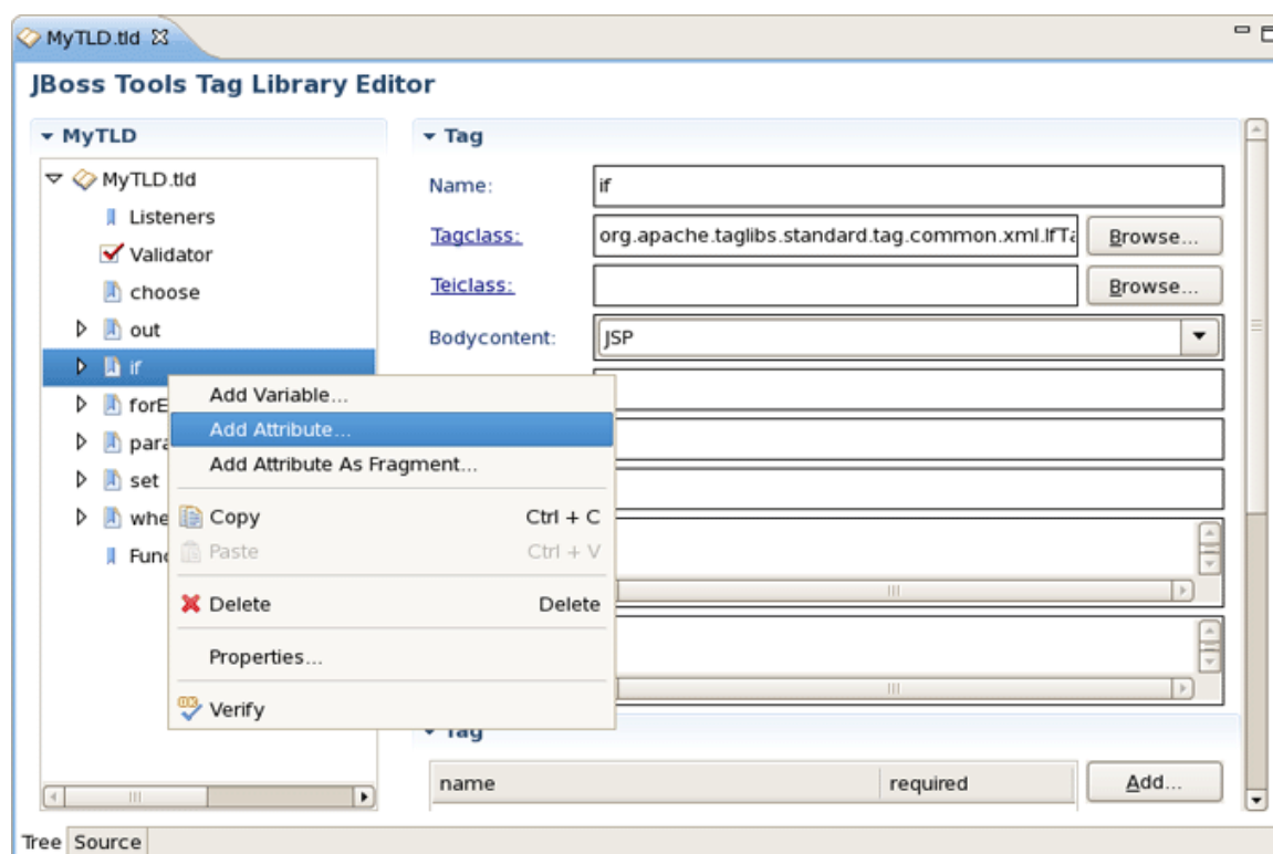
Figure 3.76. Adding a New Attribute
