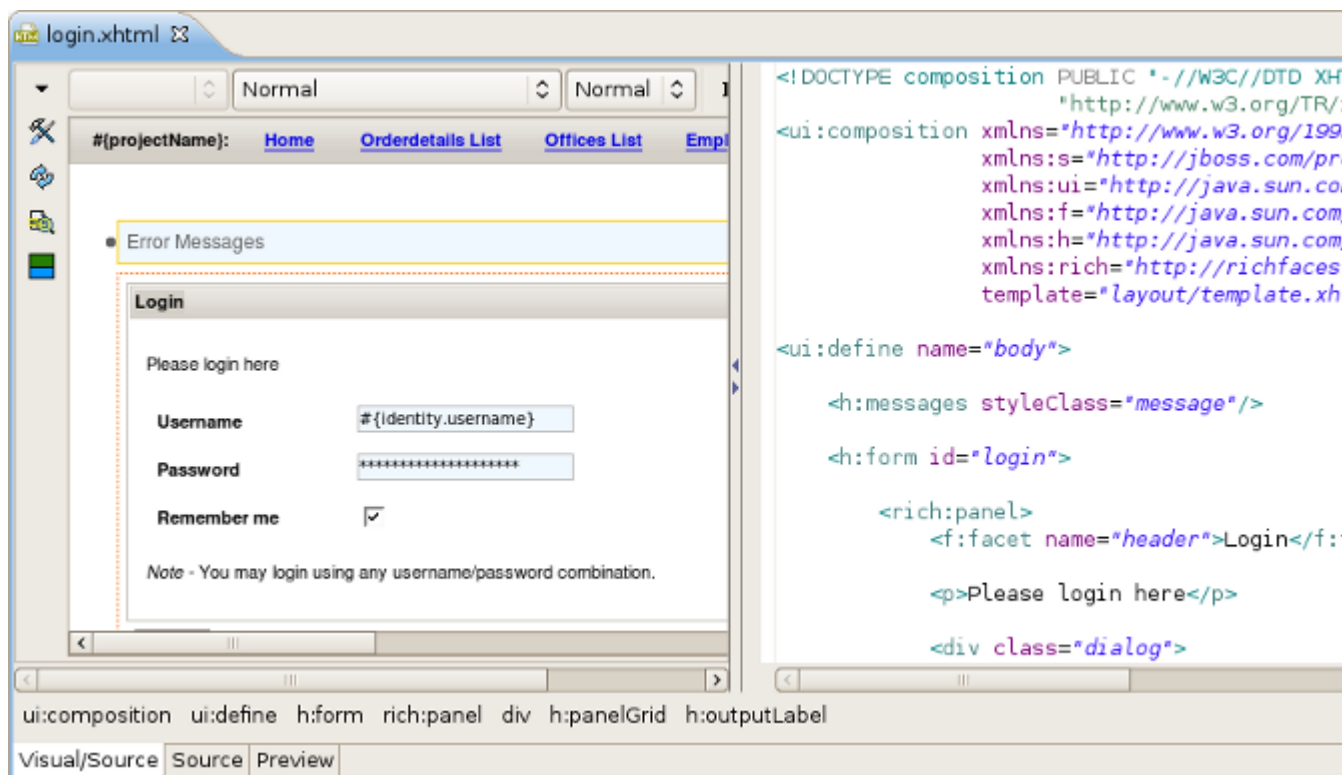
Figure 3.67. Visual Page Editor After Layout Changing
