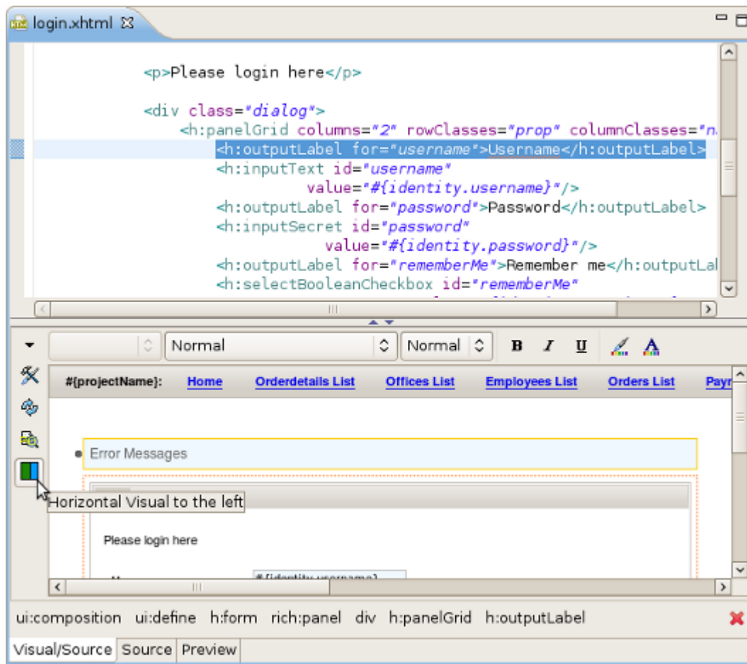
Figure 3.66. Visual Page Editor Before Layout Changing
