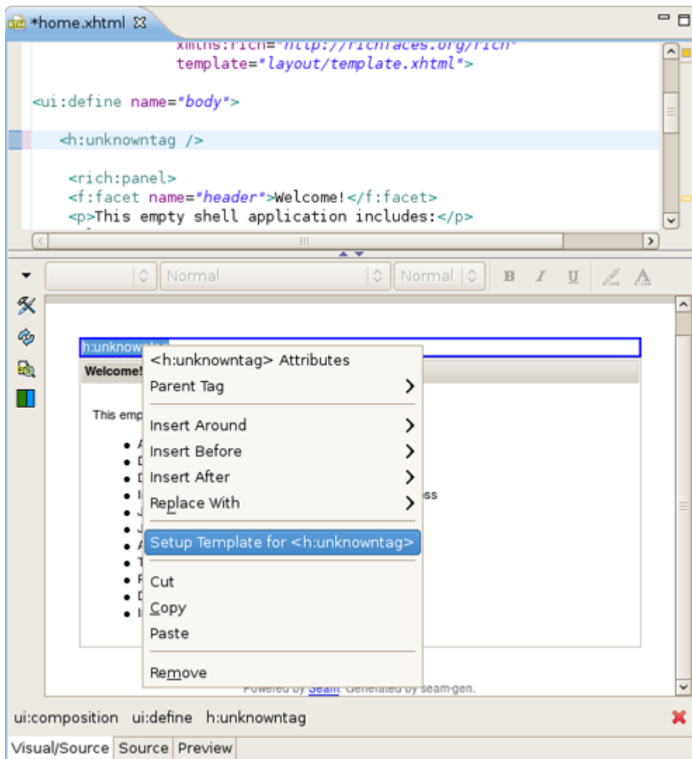
Figure 3.54. Calling Template Dialog
