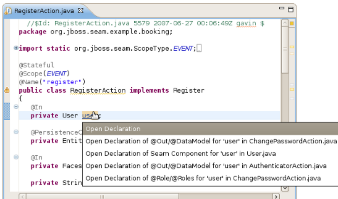
Figure 7.17. OpenOn in Seam Component
