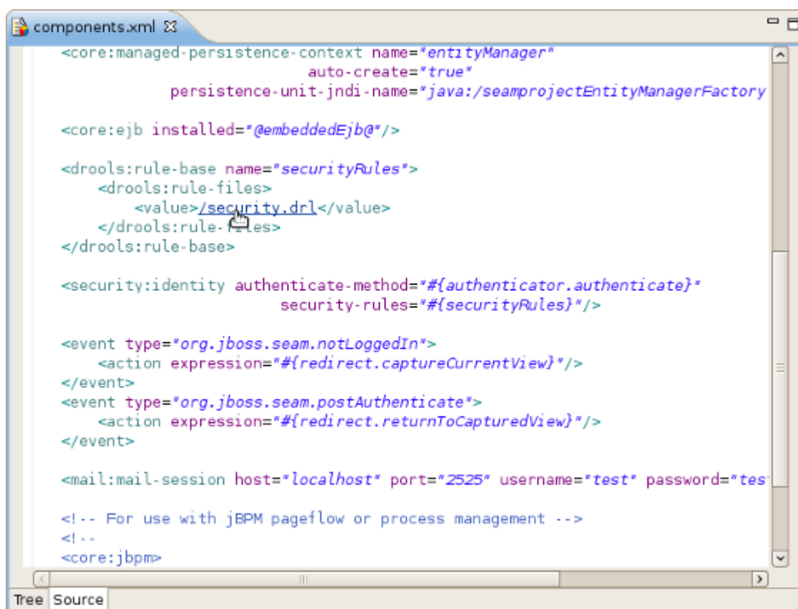
Figure 7.14. OpenOn in components.xml file
