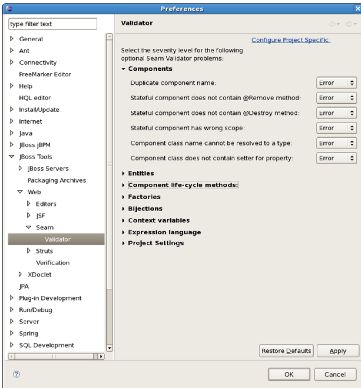
Figure 7.19. Seam Validator Preferences
