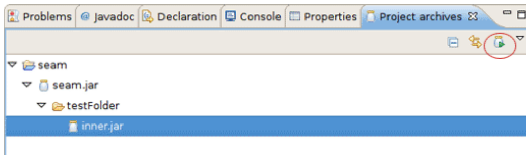
Figure 3.26. Archives View
