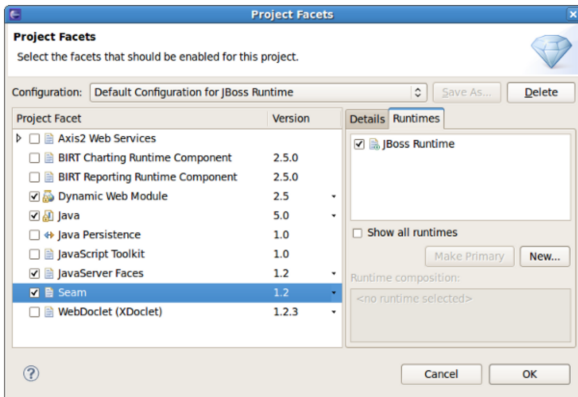
Figure 4.5. Runtimes on the Project Facets Wizard
