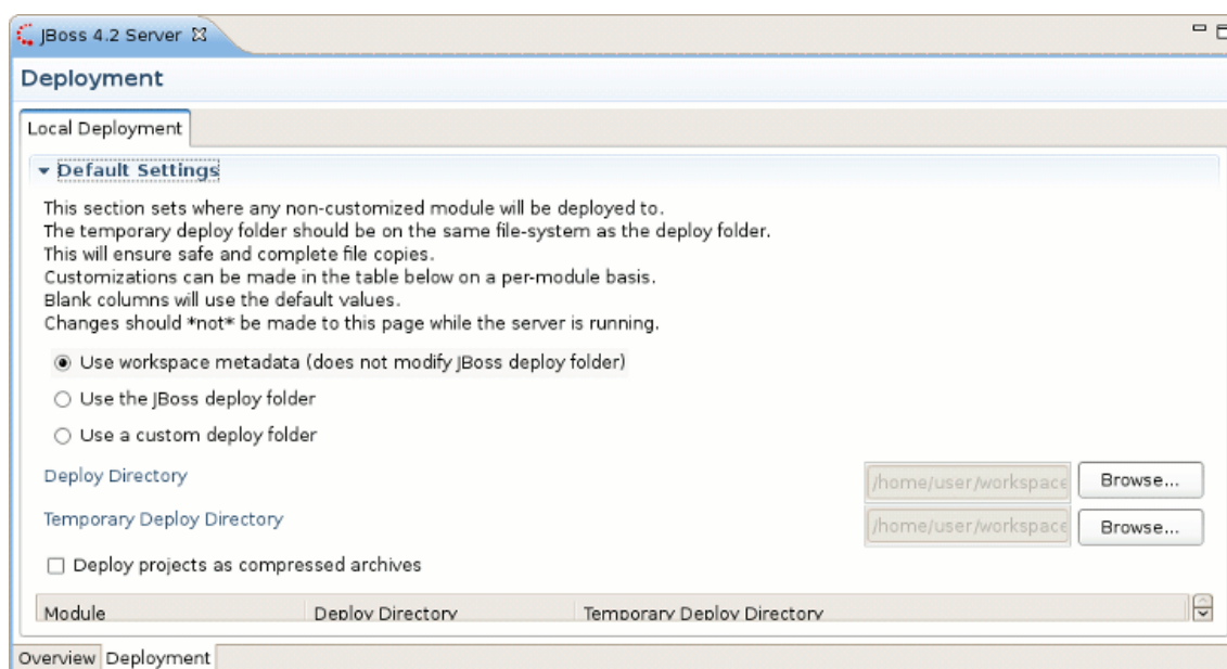
Figure 3.25. Deployment tab
