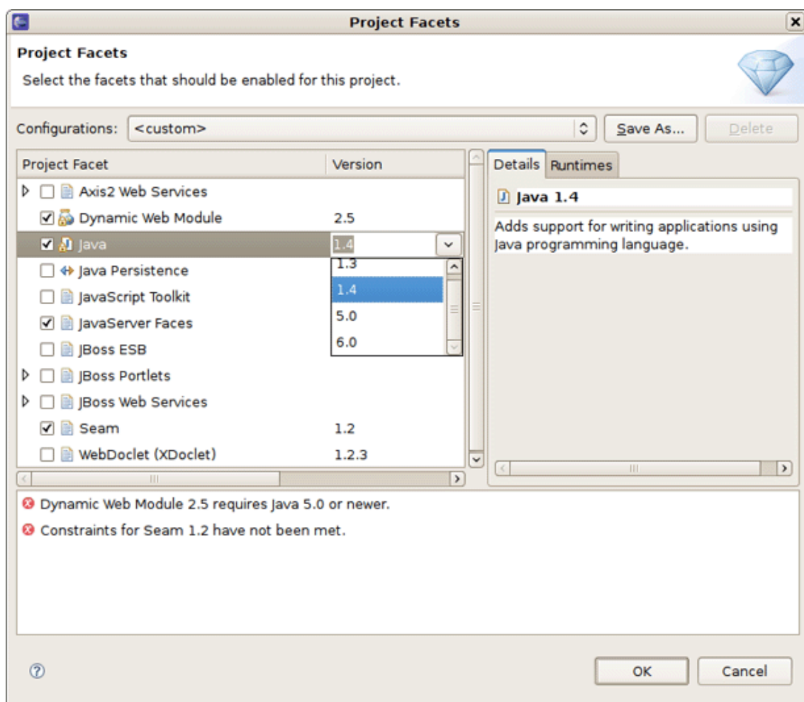
Figure 4.4. Facet Constraints
