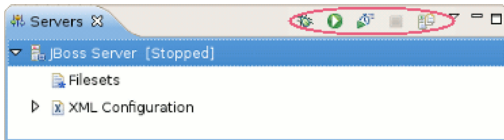
Figure 1.1. Servers Toolbar
