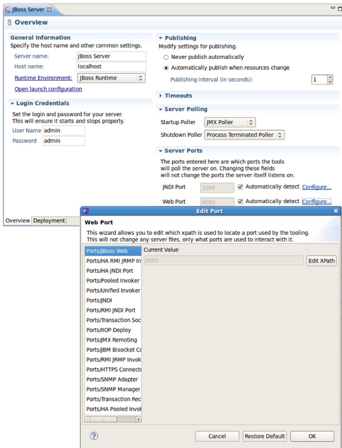
Figure 3.21. Server Ports Preferences
