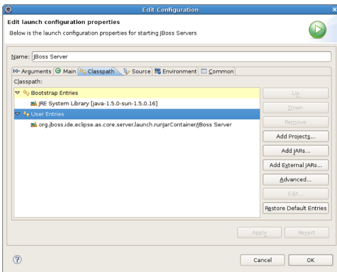
Figure 3.24. Server Classpaths
