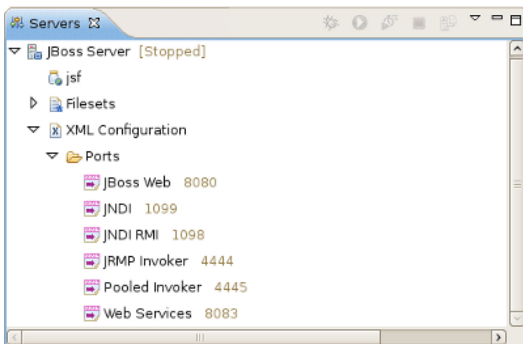
Figure 3.12. XML Configuration
