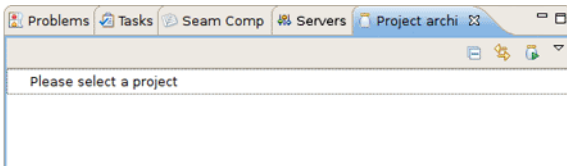
Figure 3.27. Archives View
