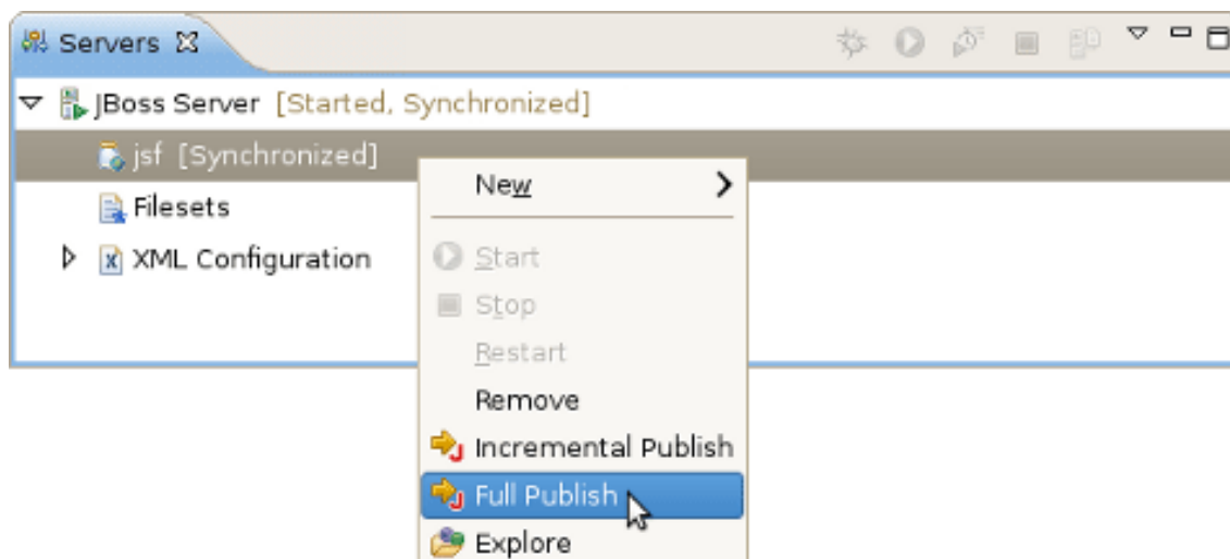
Figure 5.6. Full Publish
