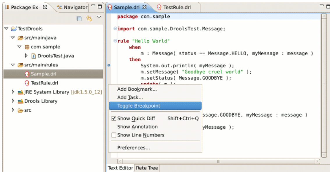
Figure 3.1. Adding Breakpoints
