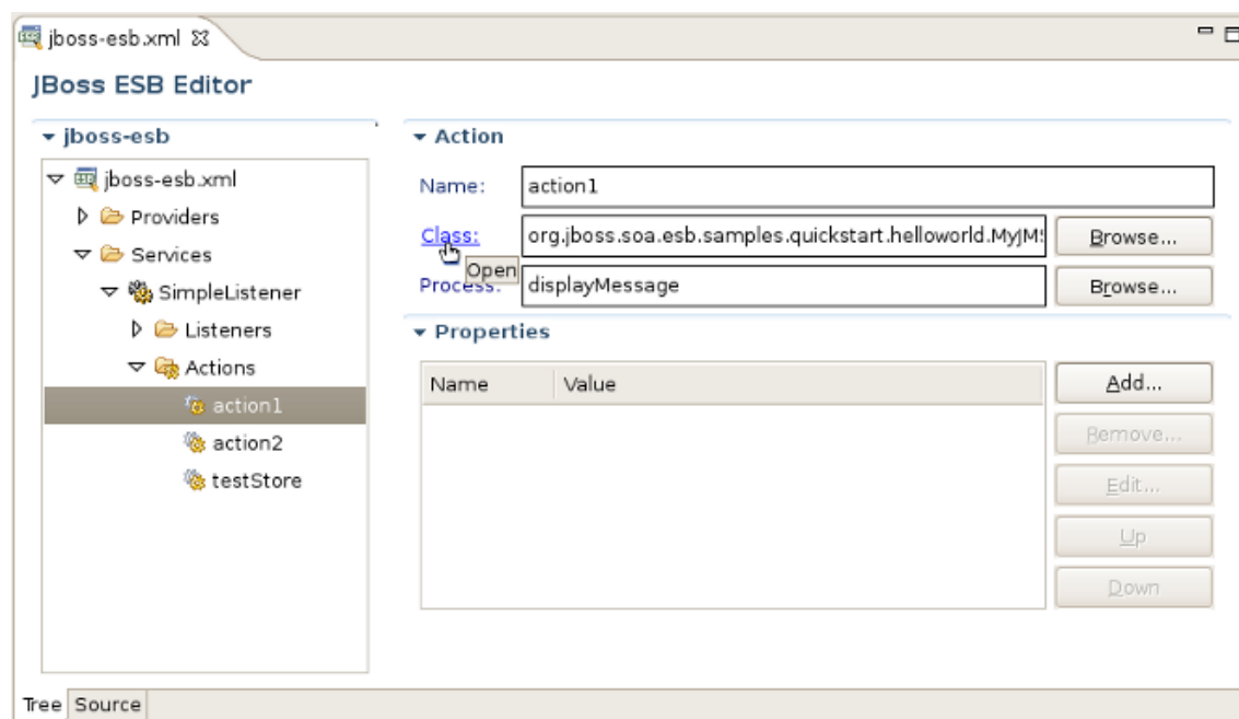
Figure 3.4. Property Link to the Associated Editor
