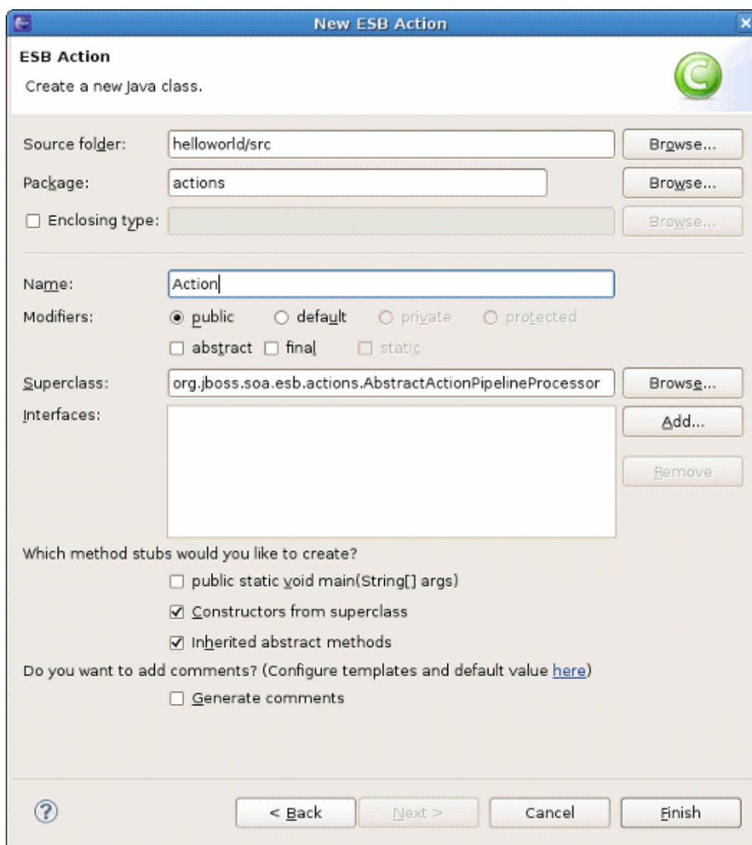
Figure 2.19. New ESB Action wizard
