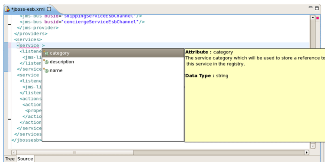
Figure 3.18. Content Assist for attributes
