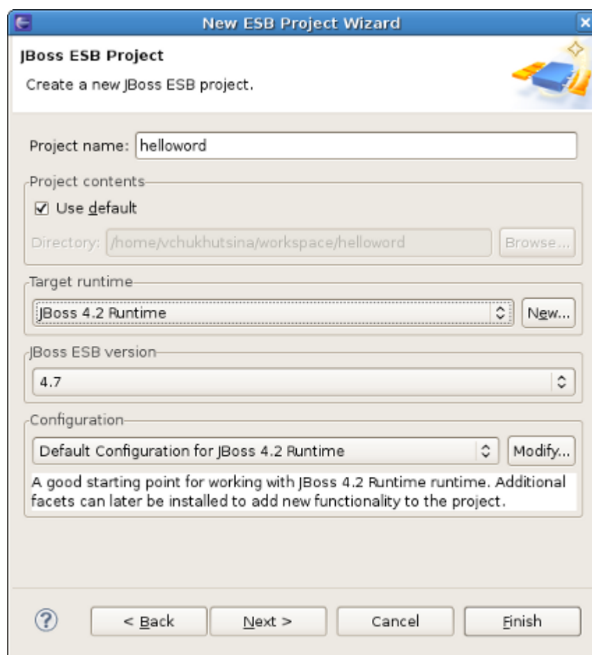
Figure 2.2. JBoss ESB Project wizard
