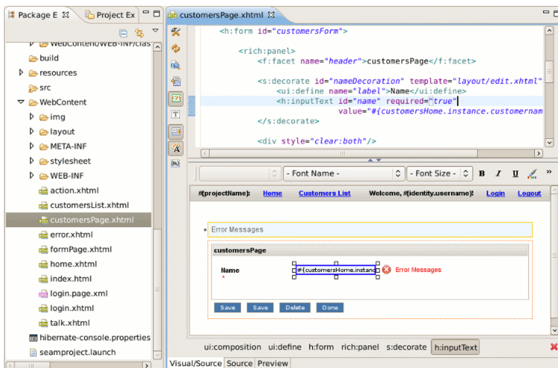
Figure 6.18. Entity Page in JBoss Tools HTML Editor.
