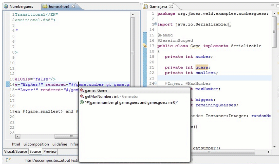
Figure 8.12. Content assist for @Named beans
