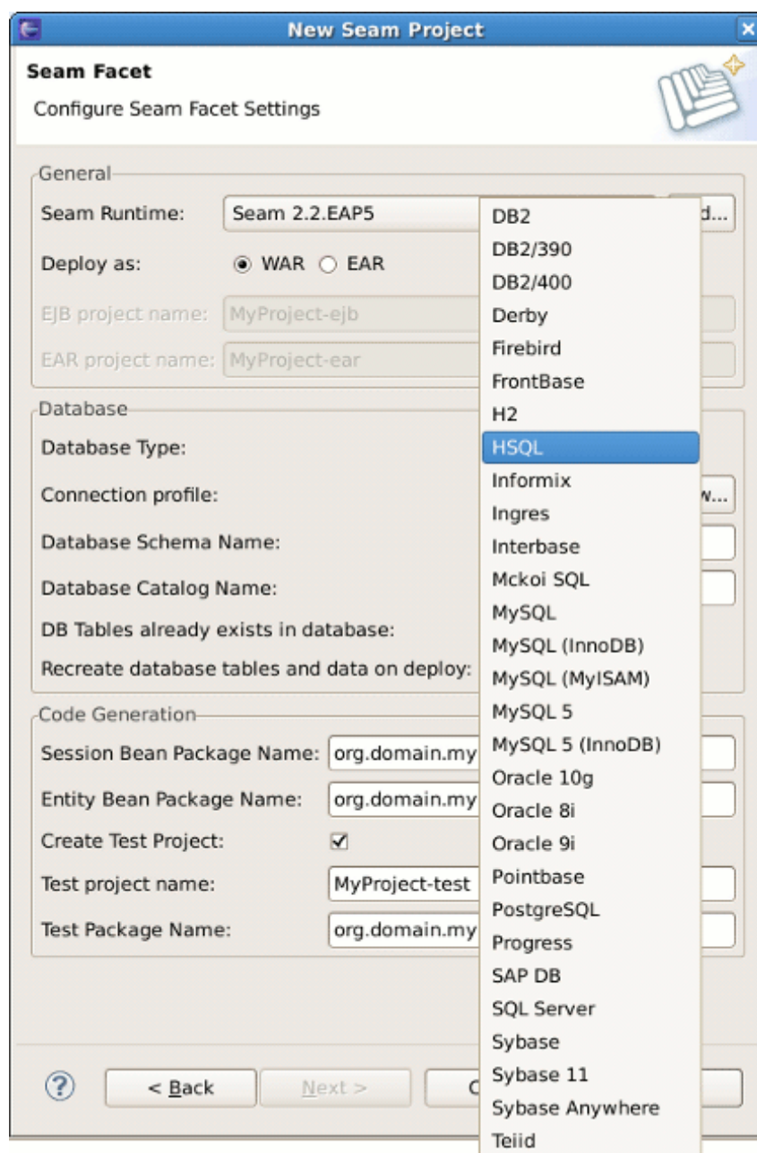
Figure 2.25. Database Type Selecting
