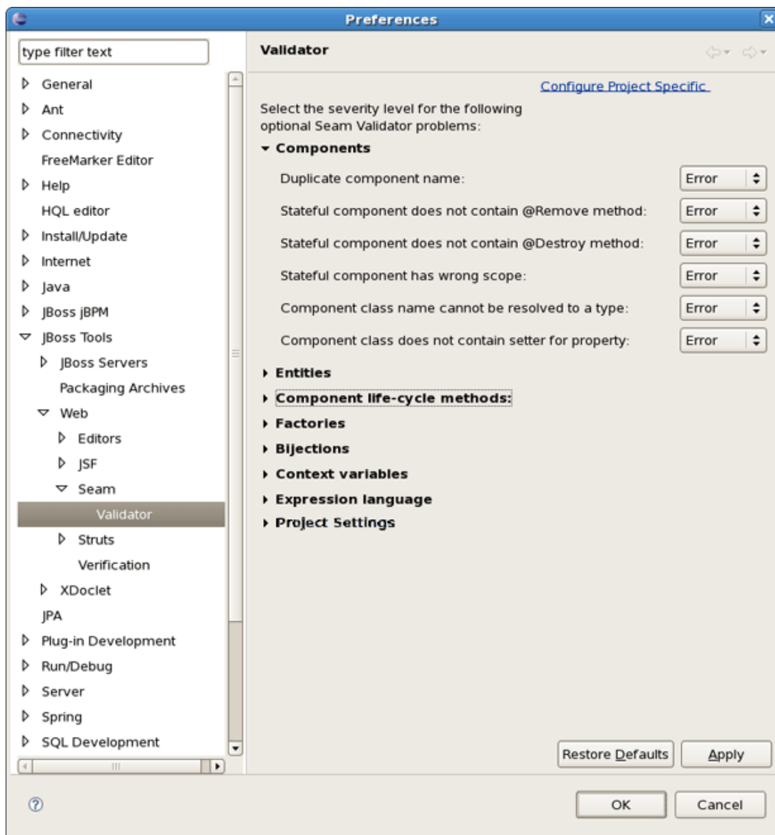
Figure 8.20. Seam Validator Preferences
