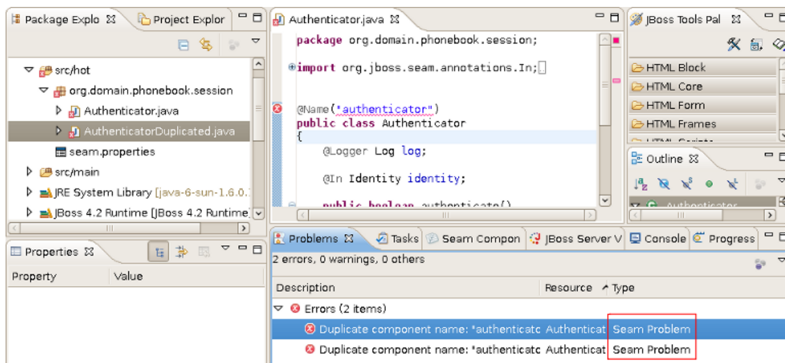
Figure 8.19. Seam Validation
