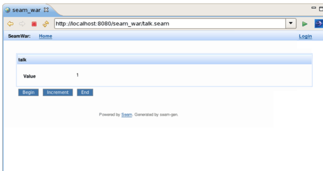
Figure 6.14. Conversation Component
