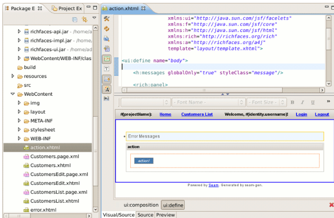
Figure 6.5. Action Page in JBoss Tools HTML Editor.
