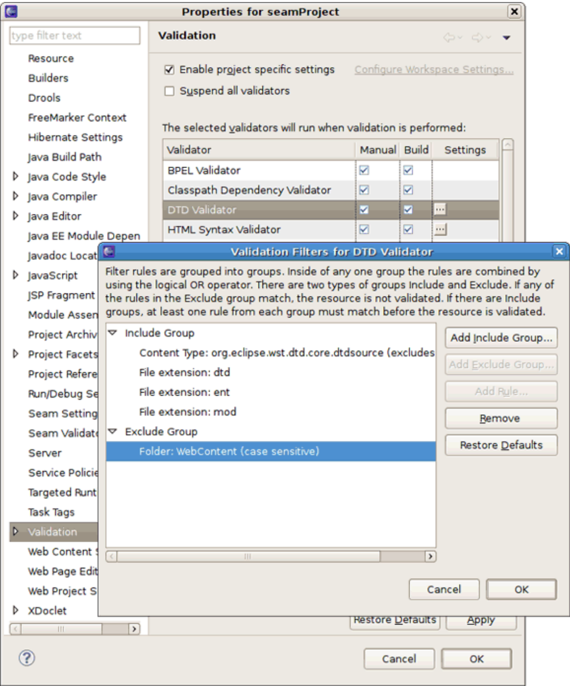
Figure 8.23. Validation Filters
