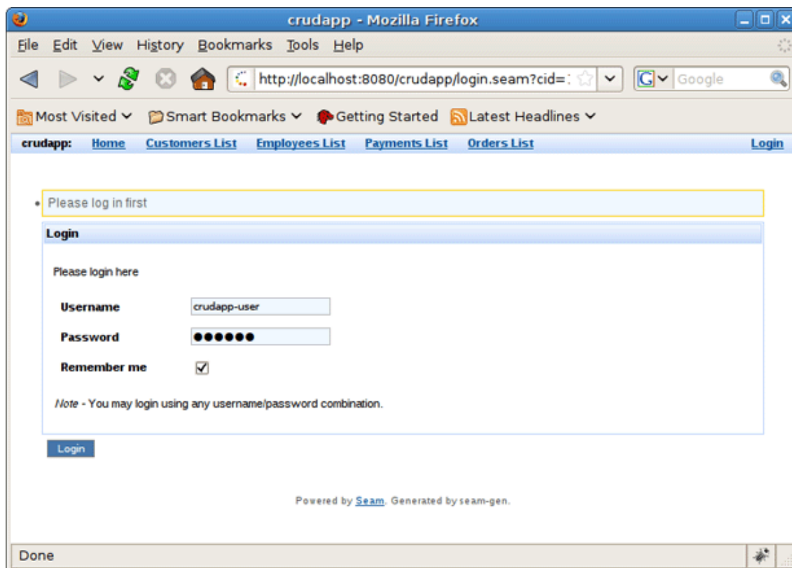
Figure 14.6. Login page
