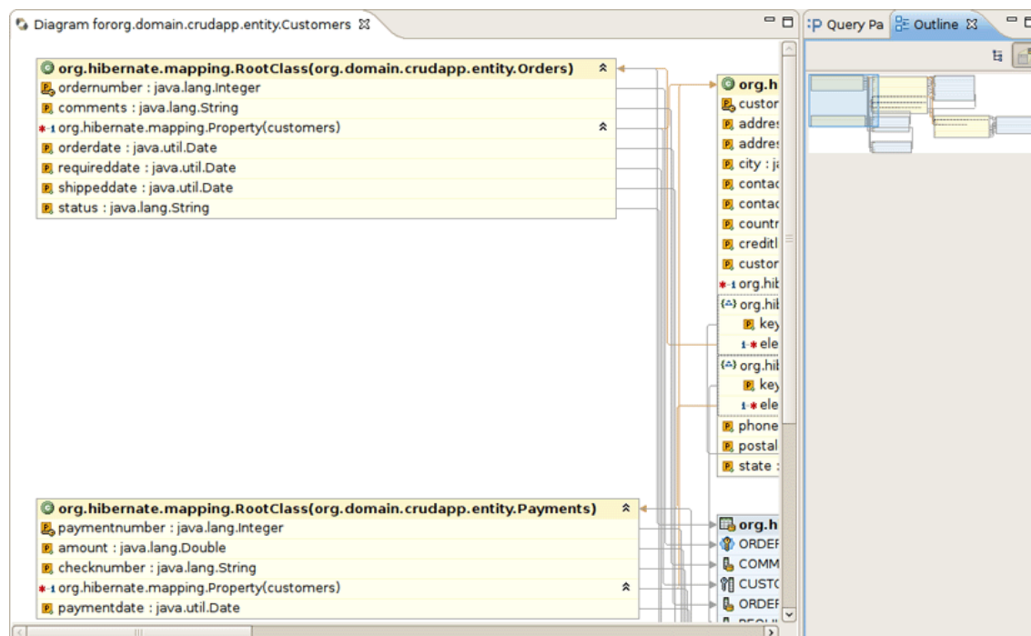
Figure 13.22. Mapping Diagram
