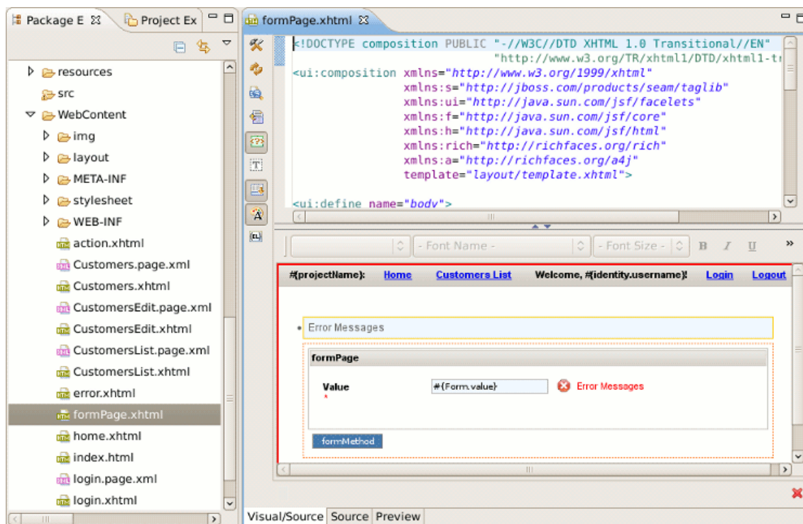
Figure 6.9. Form Page in JBoss Tools HTML Editor.
