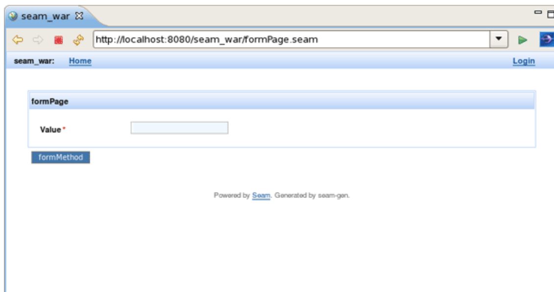
Figure 6.10. Form Component
