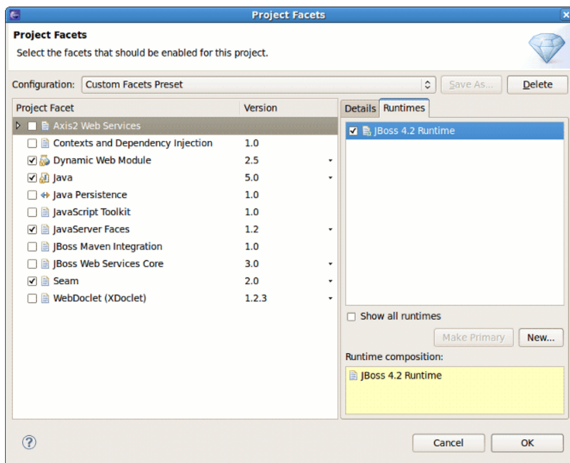
Figure 2.12. Setting Runtime
