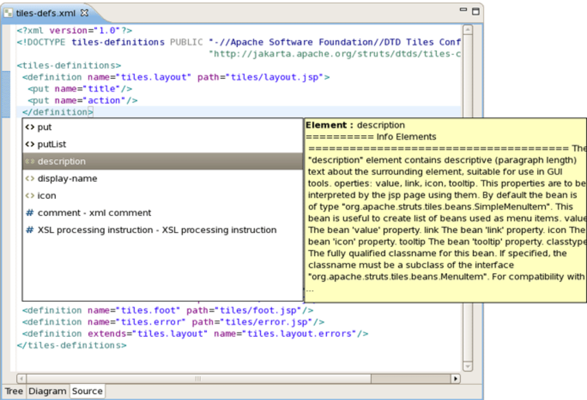
Figure 3.17. Code Assist
