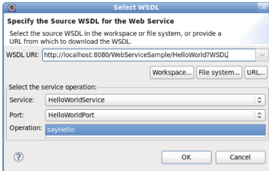
Figure 7.4. Select WSDL
