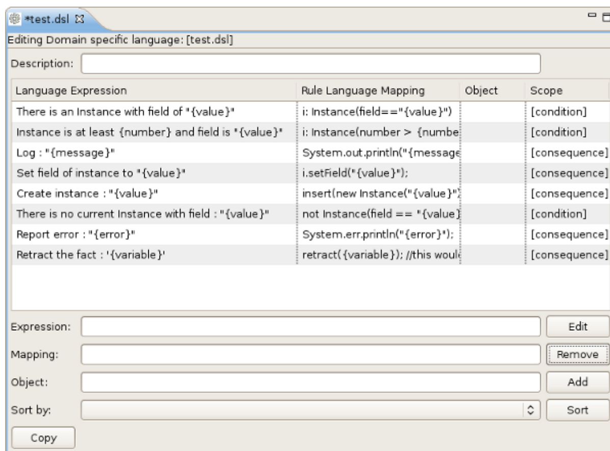
Figure 4.1. DSL Editor
