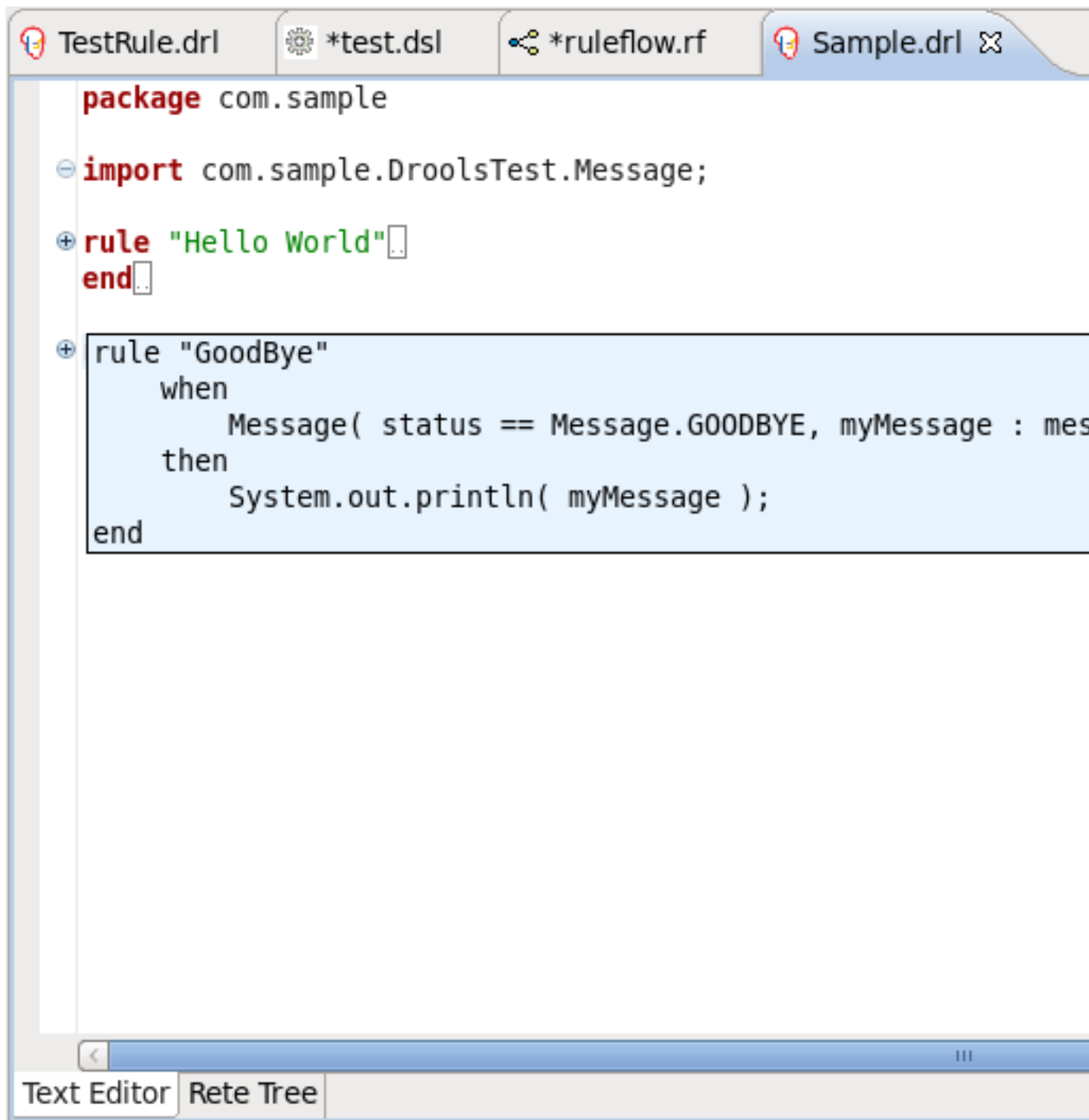
Figure 4.12. Code Folding
