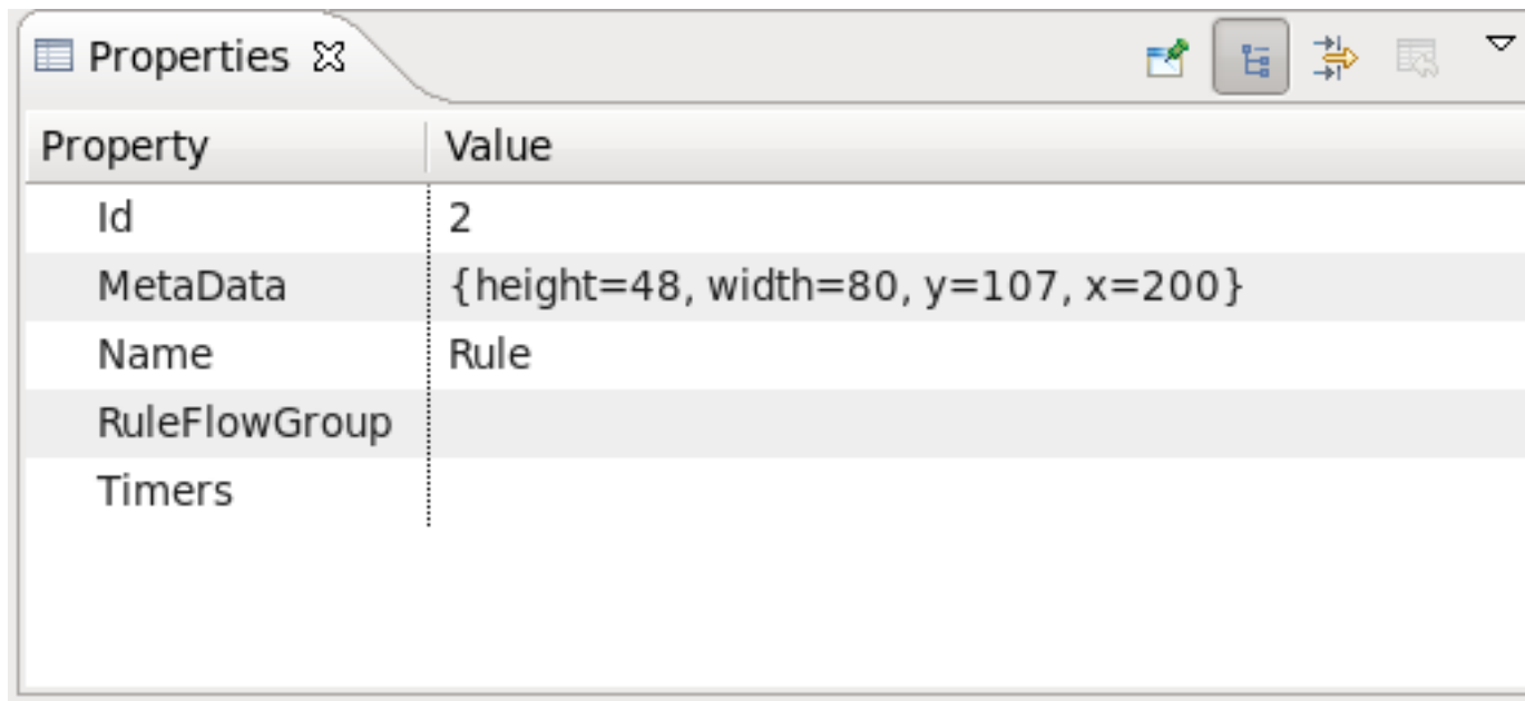
Figure 4.7. Properties view
