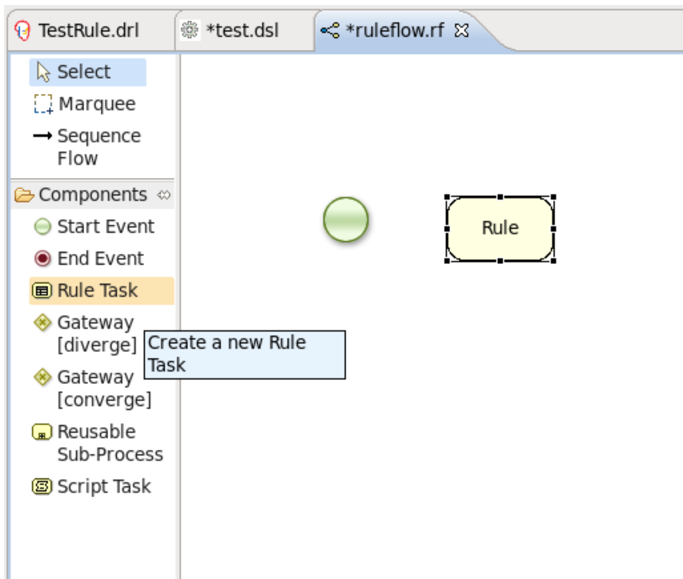
Figure 4.6. Adding an element to the canvas
