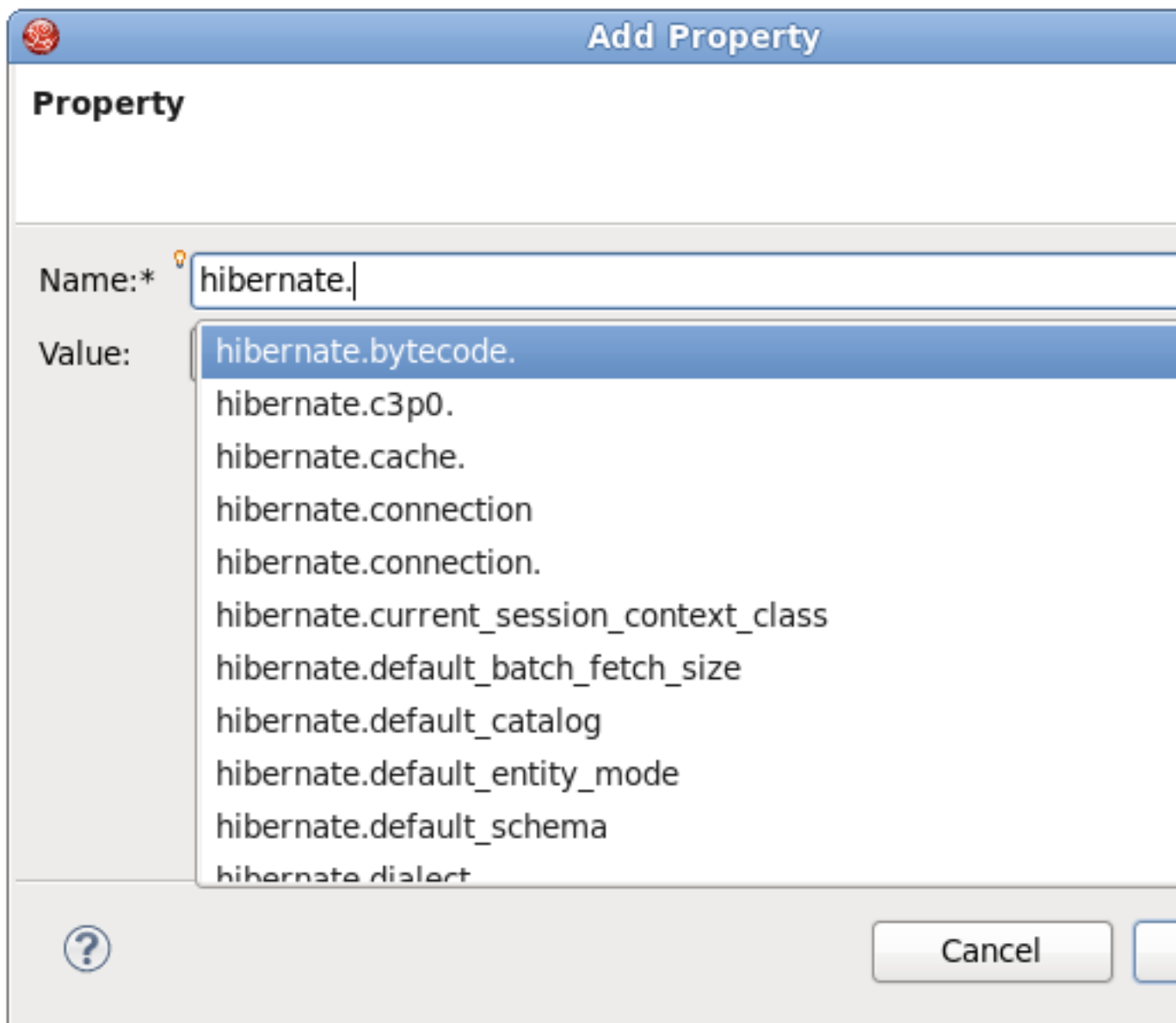
Figure 4.27. Content Assist for Properties Names
