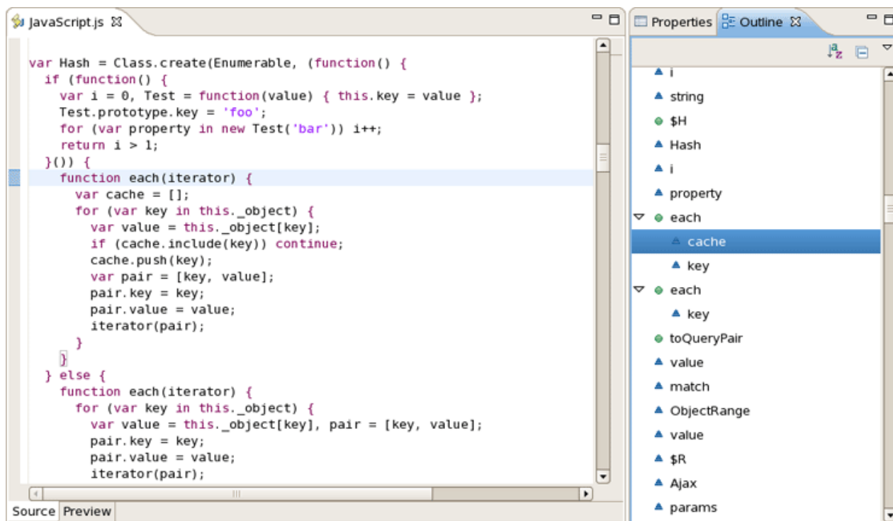
Figure 3.116. JavaScript Editor with the Outline view
