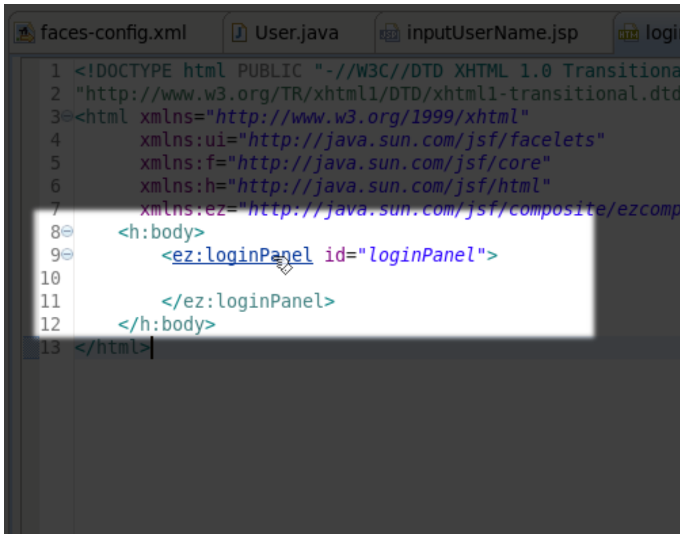
Figure 3.9. OpenOn with JSF 2.0 Component
