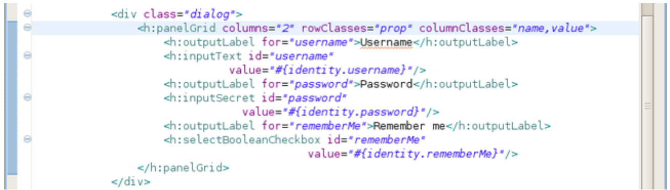
Figure 3.51. Enabled Code Folding
