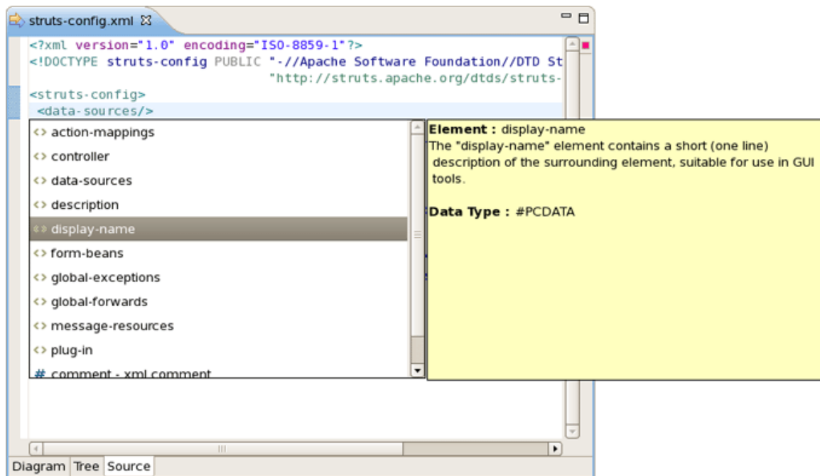
Figure 3.7. Code Assist
