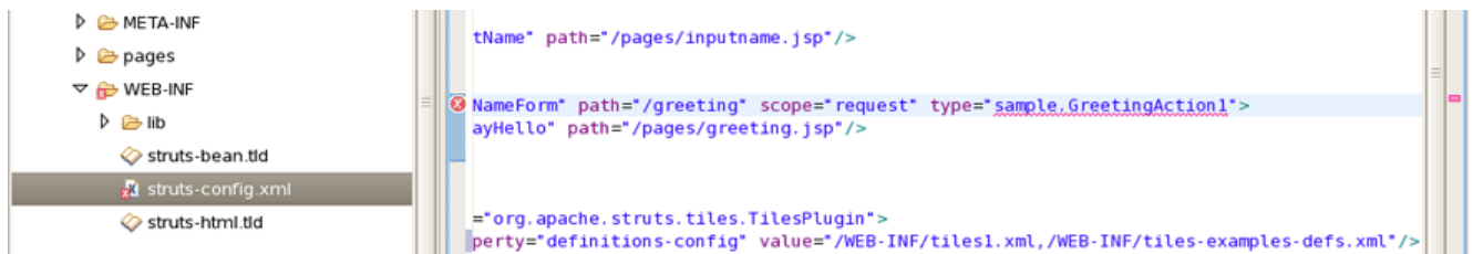
Figure 8.3. Error Reporting
