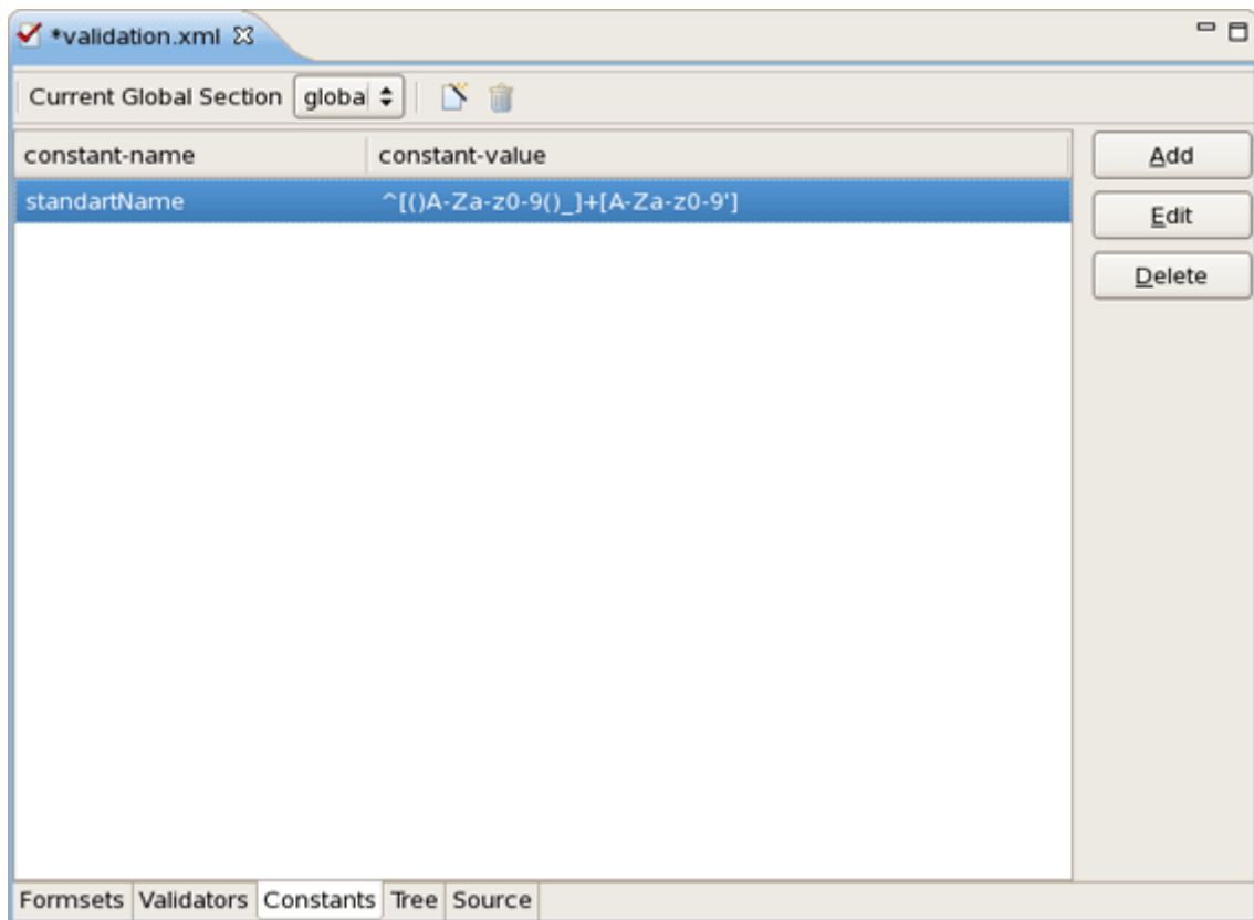
Figure 3.22. Constants View
