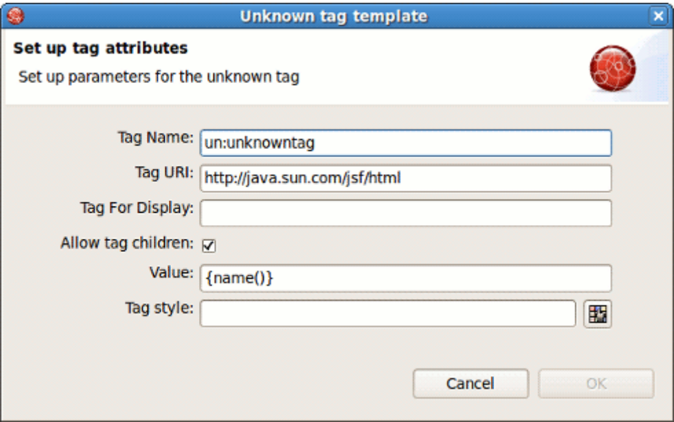
Figure 3.68. Template Dialog
